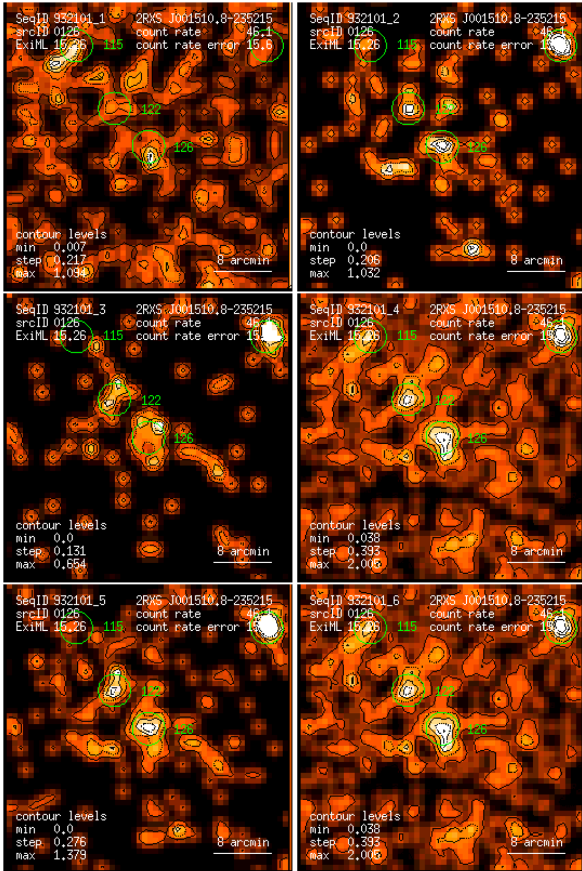
Figure 126: RASS 932101: detection 0126: band rate images, Gaussian filter: (1) PSPC channels 11 – 41, (2) 52 – 90, (3) 91 – 201, (4) 11 – 235, (5) 52 – 201, (6) 11 – 201. Broad band rates in counts/ks. Band rate contour levels in counts/ks/arcmin 2 .
