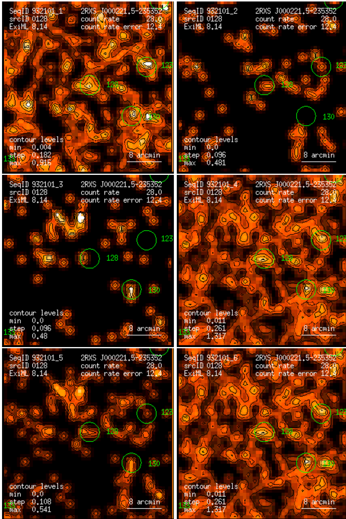
Figure 128: RASS 932101: detection 0128: band rate images, Gaussian filter: (1) PSPC channels 11 – 41, (2) 52 – 90, (3) 91 – 201, (4) 11 – 235, (5) 52 – 201, (6) 11 – 201. Broad band rates in counts/ks. Band rate contour levels in counts/ks/arcmin 2 .
