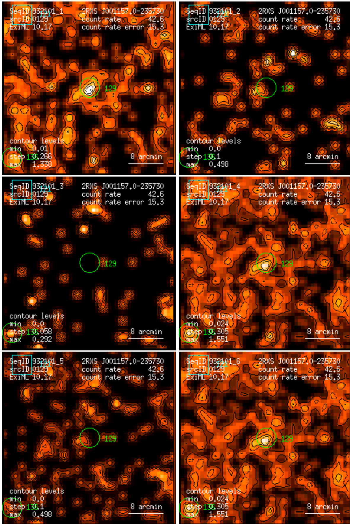
Figure 129: RASS 932101: detection 0129: band rate images, Gaussian filter: (1) PSPC channels 11 – 41, (2) 52 – 90, (3) 91 – 201, (4) 11 – 235, (5) 52 – 201, (6) 11 – 201. Broad band rates in counts/ks. Band rate contour levels in counts/ks/arcmin 2 .
