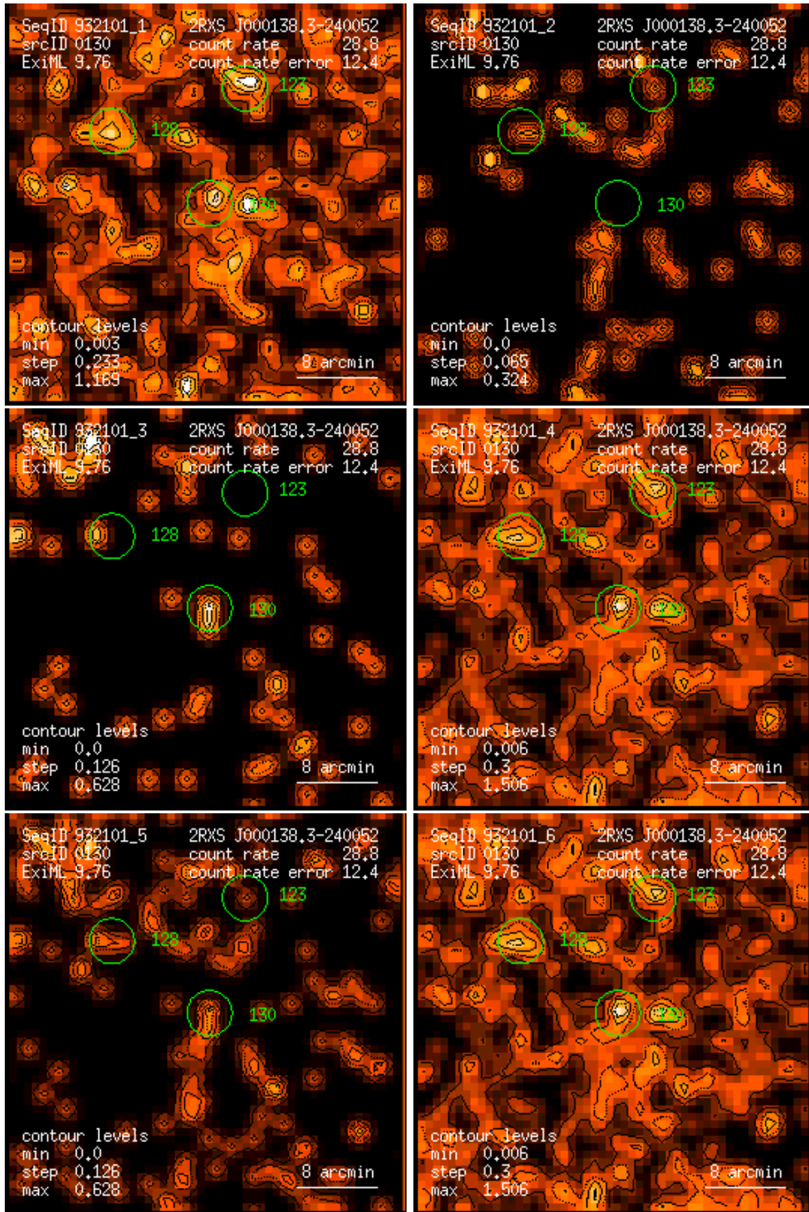
Figure 130: RASS 932101: detection 0130: band rate images, Gaussian filter: (1) PSPC channels 11 – 41, (2) 52 – 90, (3) 91 – 201, (4) 11 – 235, (5) 52 – 201, (6) 11 – 201. Broad band rates in counts/ks. Band rate contour levels in counts/ks/arcmin 2 .
