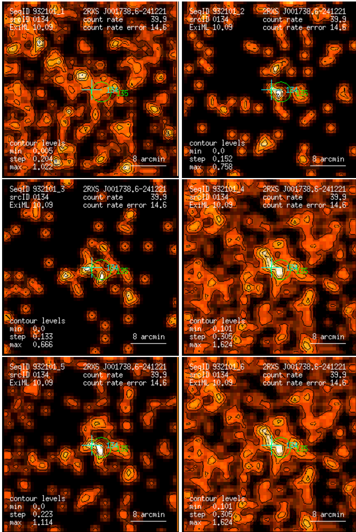
Figure 134: RASS 932101: detection 0134: band rate images, Gaussian filter: (1) PSPC channels 11 – 41, (2) 52 – 90, (3) 91 – 201, (4) 11 – 235, (5) 52 – 201, (6) 11 – 201. Broad band rates in counts/ks. Band rate contour levels in counts/ks/arcmin 2 .
