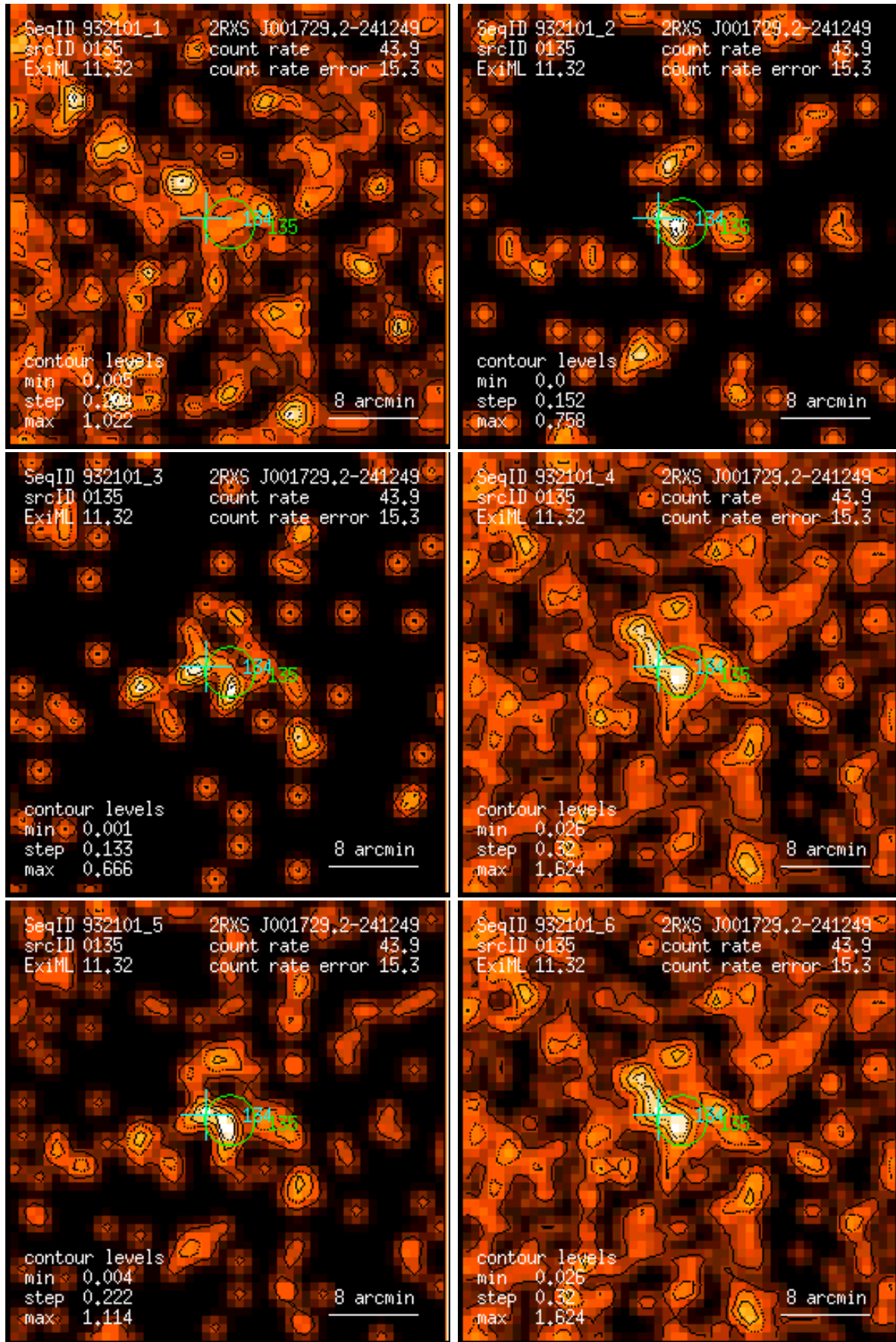
Figure 135: RASS 932101: detection 0135: band rate images, Gaussian filter: (1) PSPC channels 11 – 41, (2) 52 – 90, (3) 91 – 201, (4) 11 – 235, (5) 52 – 201, (6) 11 – 201. Broad band rates in counts/ks. Band rate contour levels in counts/ks/arcmin 2 .
