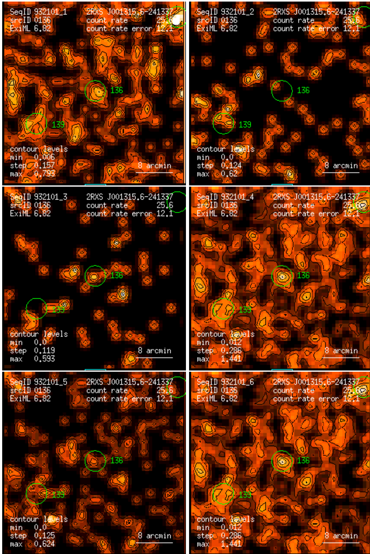
Figure 136: RASS 932101: detection 0136: band rate images, Gaussian filter: (1) PSPC channels 11 – 41, (2) 52 – 90, (3) 91 – 201, (4) 11 – 235, (5) 52 – 201, (6) 11 – 201. Broad band rates in counts/ks. Band rate contour levels in counts/ks/arcmin 2 .
