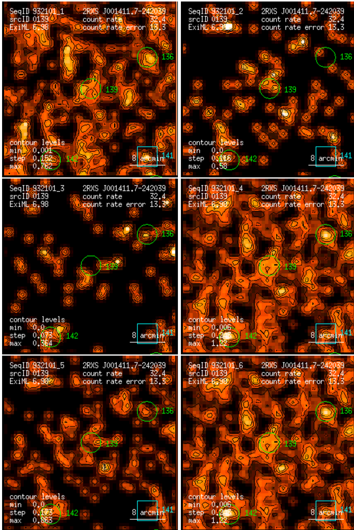
Figure 139: RASS 932101: detection 0139: band rate images, Gaussian filter: (1) PSPC channels 11 – 41, (2) 52 – 90, (3) 91 – 201, (4) 11 – 235, (5) 52 – 201, (6) 11 – 201. Broad band rates in counts/ks. Band rate contour levels in counts/ks/arcmin 2 .
