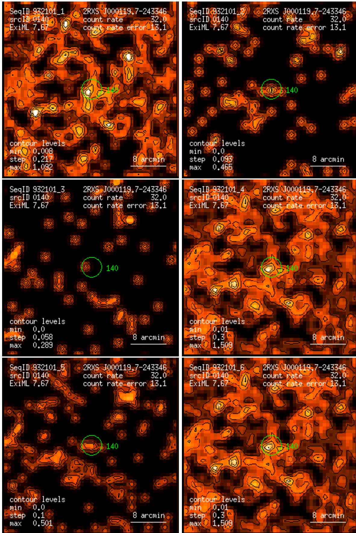
Figure 140: RASS 932101: detection 0140: band rate images, Gaussian filter: (1) PSPC channels 11 – 41, (2) 52 – 90, (3) 91 – 201, (4) 11 – 235, (5) 52 – 201, (6) 11 – 201. Broad band rates in counts/ks. Band rate contour levels in counts/ks/arcmin 2 .
