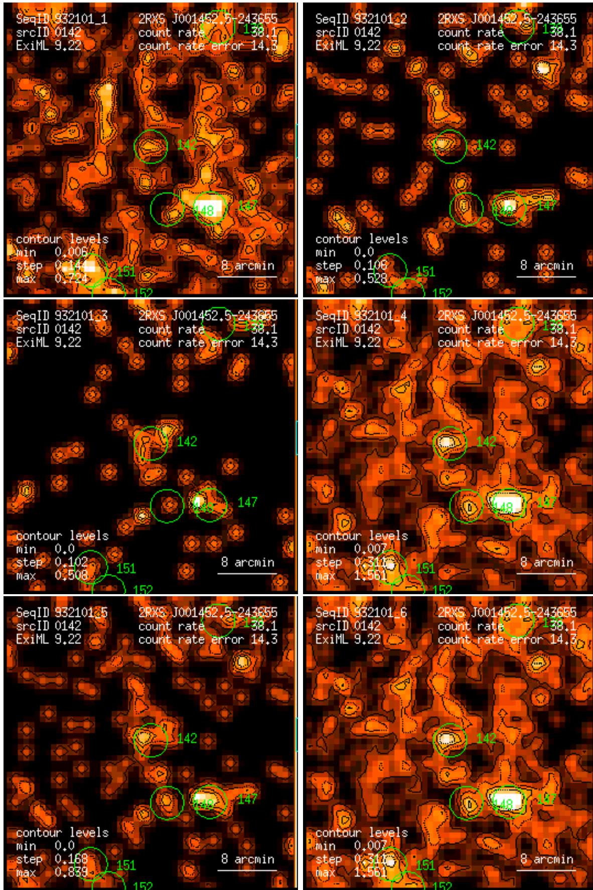
Figure 142: RASS 932101: detection 0142: band rate images, Gaussian filter: (1) PSPC channels 11 – 41, (2) 52 – 90, (3) 91 – 201, (4) 11 – 235, (5) 52 – 201, (6) 11 – 201. Broad band rates in counts/ks. Band rate contour levels in counts/ks/arcmin 2 .
