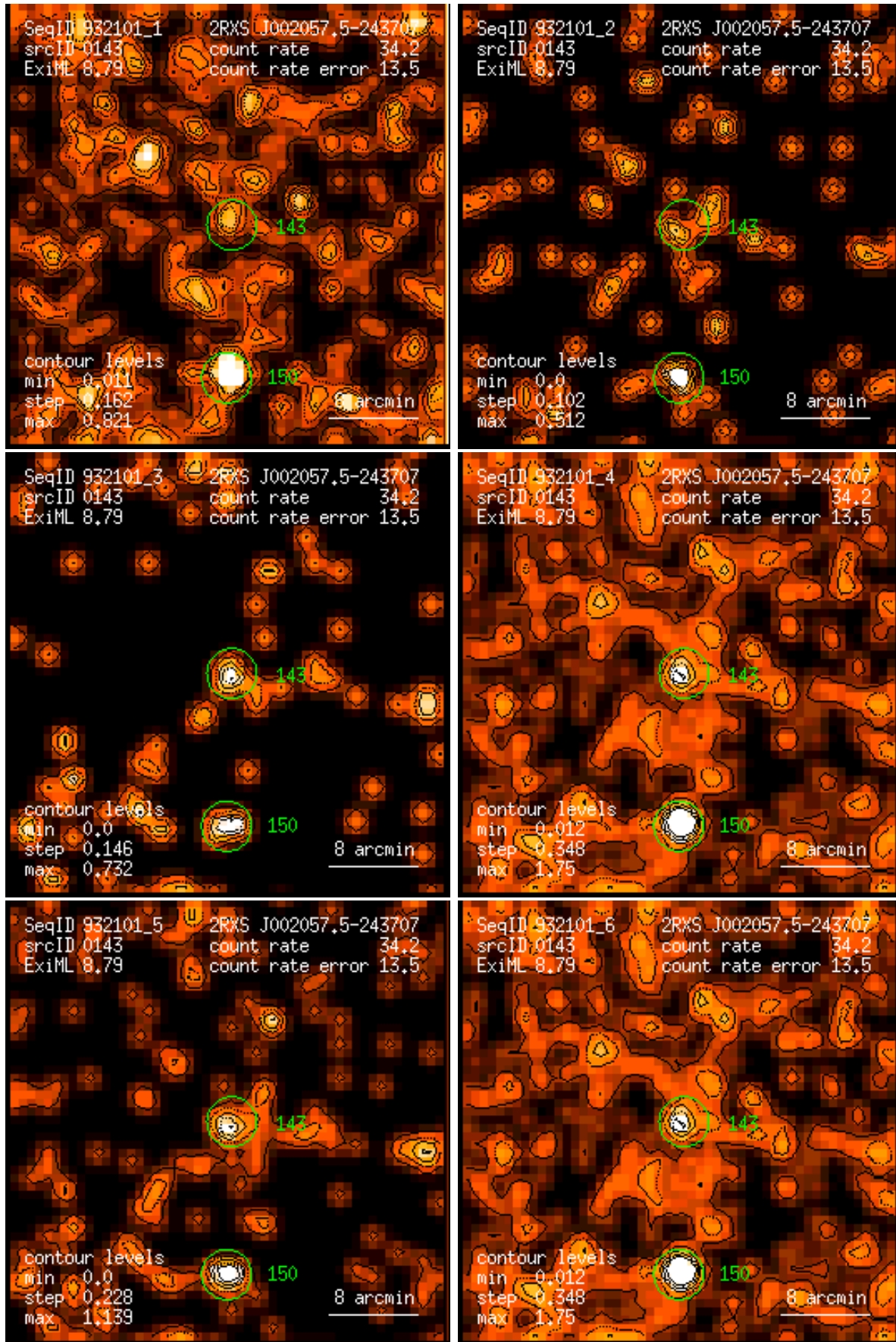
Figure 143: RASS 932101: detection 0143: band rate images, Gaussian filter: (1) PSPC channels 11 – 41, (2) 52 – 90, (3) 91 – 201, (4) 11 – 235, (5) 52 – 201, (6) 11 – 201. Broad band rates in counts/ks. Band rate contour levels in counts/ks/arcmin 2 .
