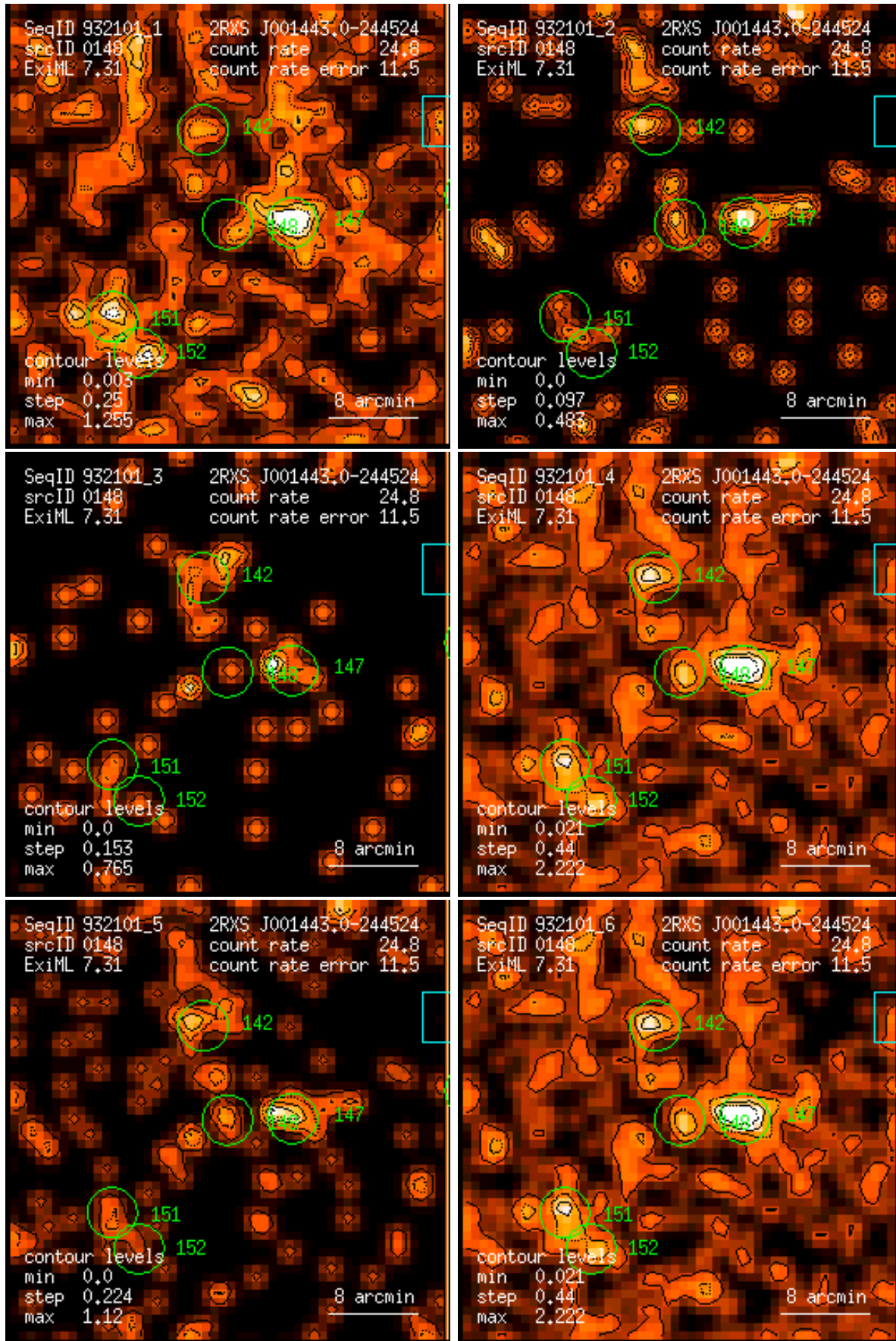
Figure 148: RASS 932101: detection 0148: band rate images, Gaussian filter: (1) PSPC channels 11 – 41, (2) 52 – 90, (3) 91 – 201, (4) 11 – 235, (5) 52 – 201, (6) 11 – 201. Broad band rates in counts/ks. Band rate contour levels in counts/ks/arcmin 2 .
