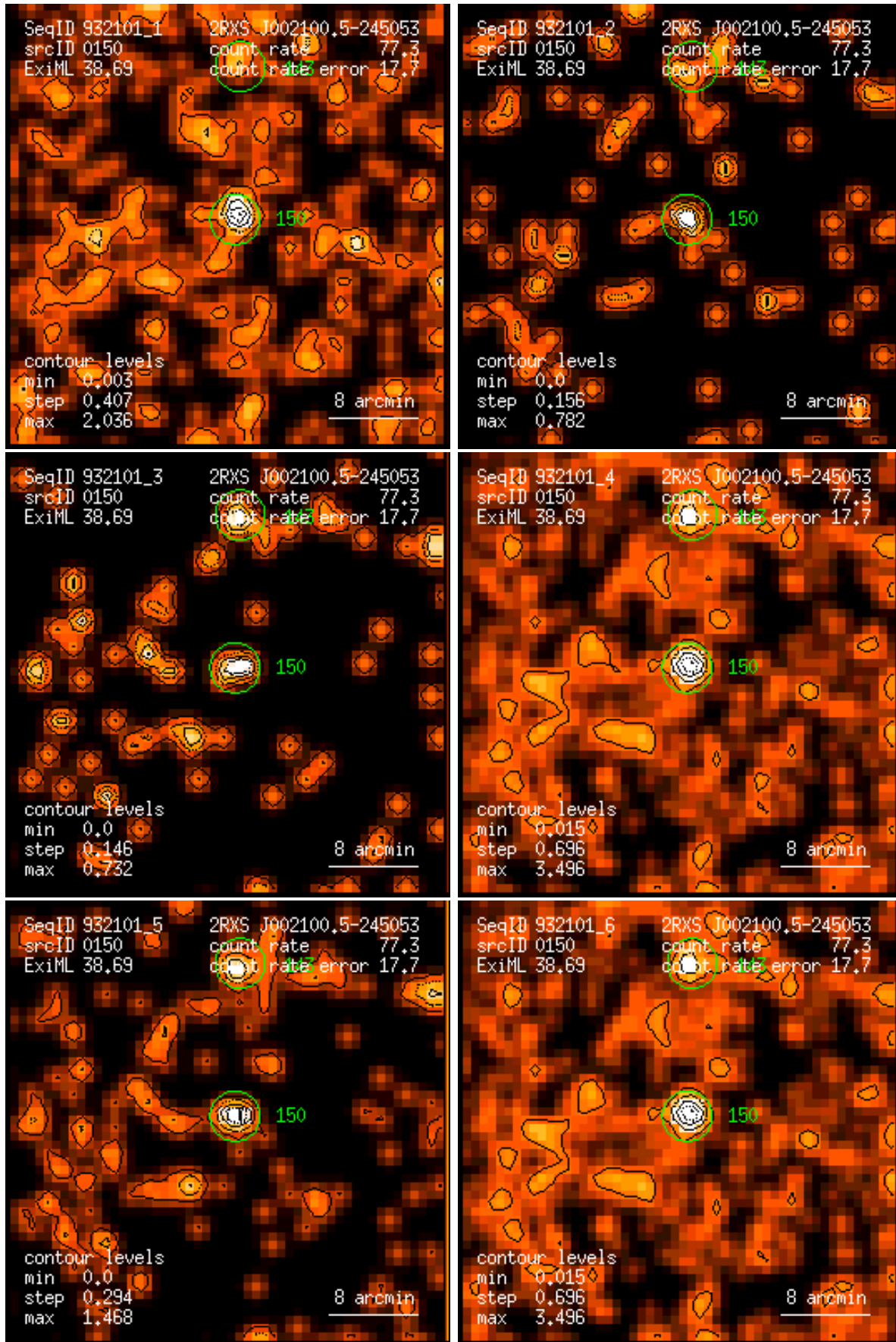
Figure 150: RASS 932101: detection 0150: band rate images, Gaussian filter: (1) PSPC channels 11 – 41, (2) 52 – 90, (3) 91 – 201, (4) 11 – 235, (5) 52 – 201, (6) 11 – 201. Broad band rates in counts/ks. Band rate contour levels in counts/ks/arcmin 2 .
