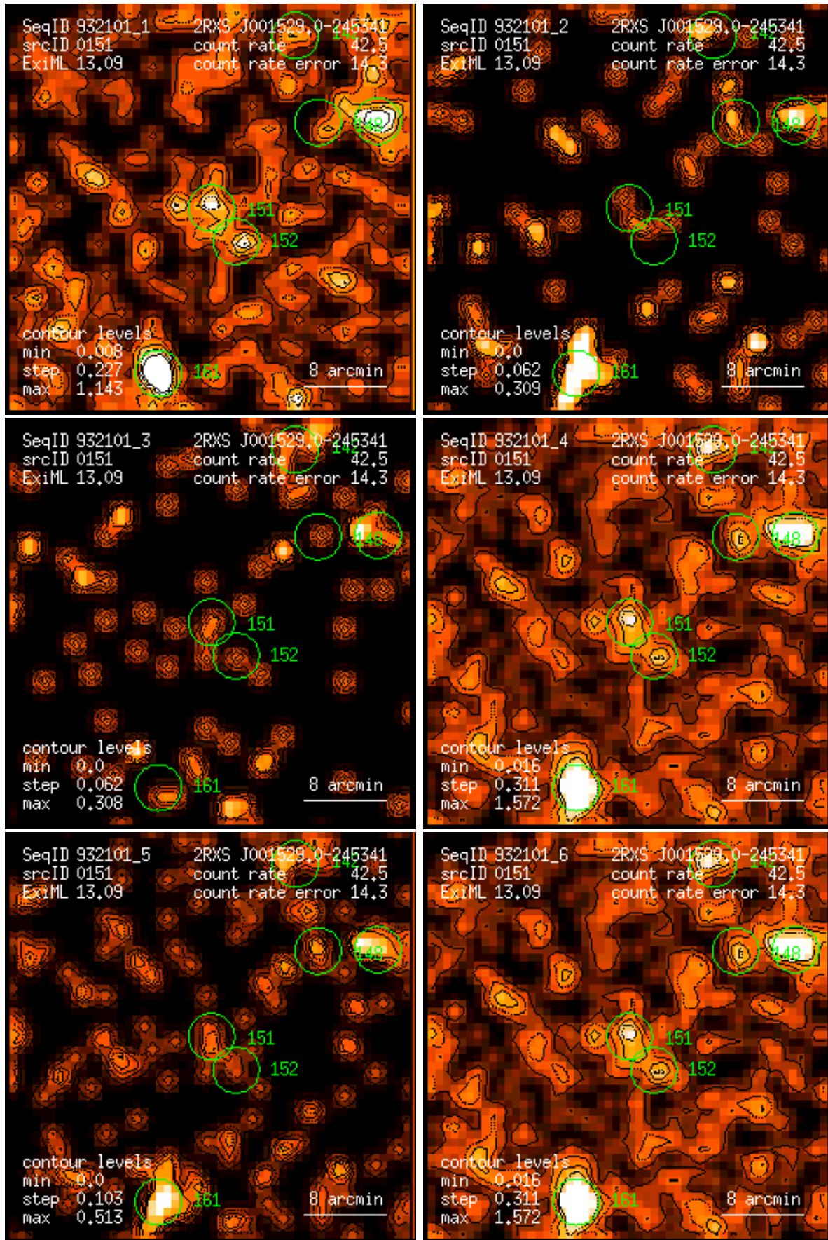
Figure 151: RASS 932101: detection 0151: band rate images, Gaussian filter: (1) PSPC channels 11 – 41, (2) 52 – 90, (3) 91 – 201, (4) 11 – 235, (5) 52 – 201, (6) 11 – 201. Broad band rates in counts/ks. Band rate contour levels in counts/ks/arcmin 2 .
