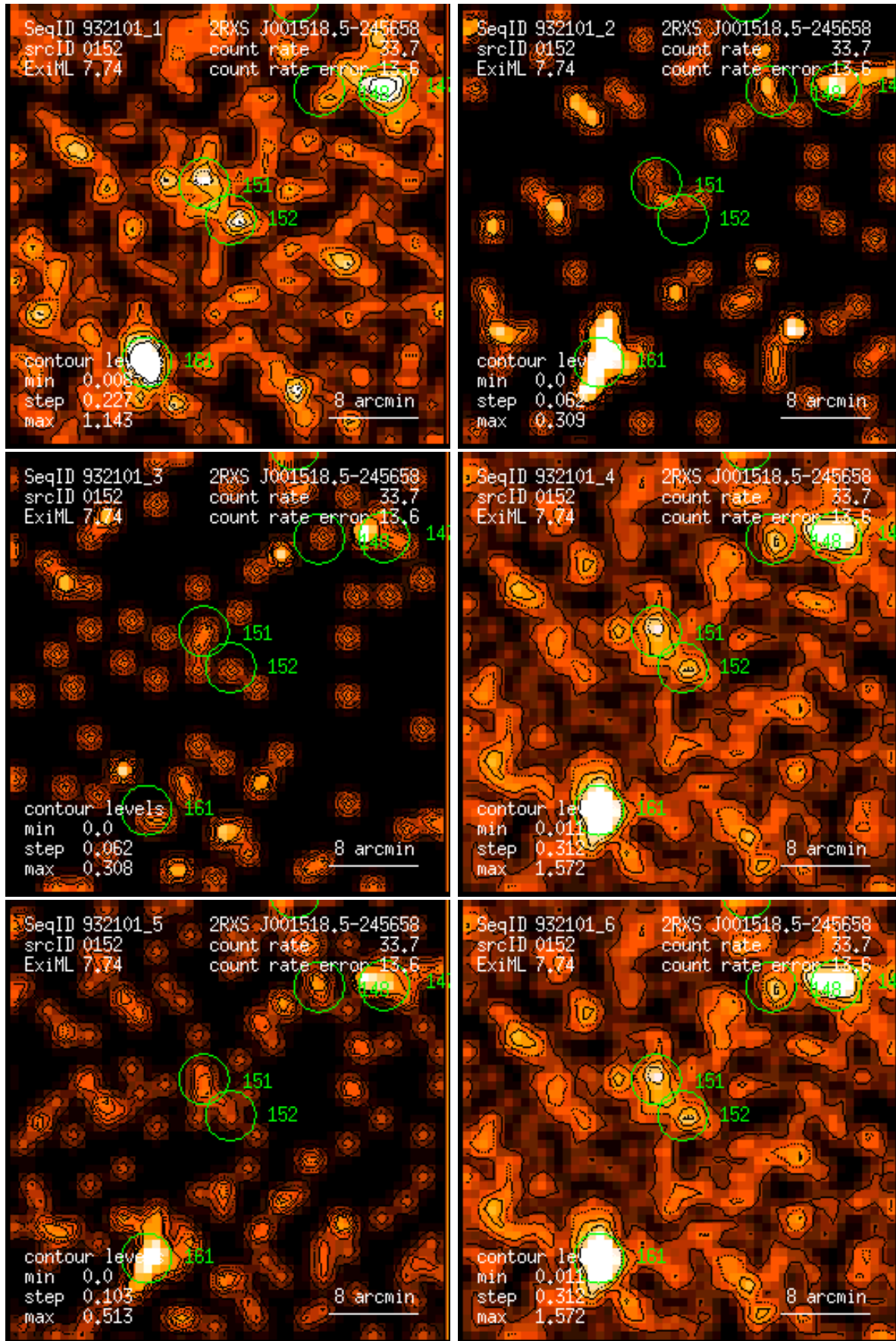
Figure 152: RASS 932101: detection 0152: band rate images, Gaussian filter: (1) PSPC channels 11 – 41, (2) 52 – 90, (3) 91 – 201, (4) 11 – 235, (5) 52 – 201, (6) 11 – 201. Broad band rates in counts/ks. Band rate contour levels in counts/ks/arcmin 2 .
