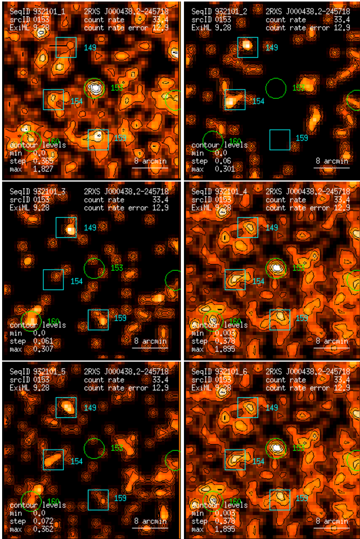
Figure 153: RASS 932101: detection 0153: band rate images, Gaussian filter: (1) PSPC channels 11 – 41, (2) 52 – 90, (3) 91 – 201, (4) 11 – 235, (5) 52 – 201, (6) 11 – 201. Broad band rates in counts/ks. Band rate contour levels in counts/ks/arcmin 2 .
