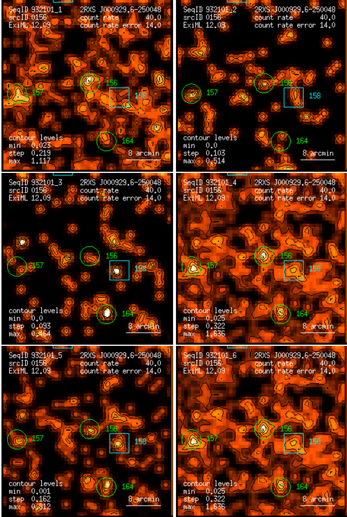
Figure 156: RASS 932101: detection 0156: band rate images, Gaussian filter: (1) PSPC channels 11 – 41, (2) 52 – 90, (3) 91 – 201, (4) 11 – 235, (5) 52 – 201, (6) 11 – 201. Broad band rates in counts/ks. Band rate contour levels in counts/ks/arcmin 2 .
