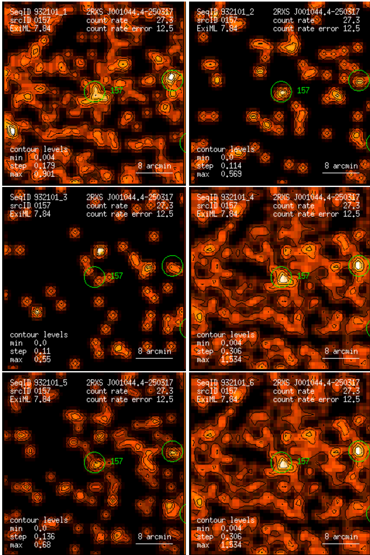
Figure 157: RASS 932101: detection 0157: band rate images, Gaussian filter: (1) PSPC channels 11 – 41, (2) 52 – 90, (3) 91 – 201, (4) 11 – 235, (5) 52 – 201, (6) 11 – 201. Broad band rates in counts/ks. Band rate contour levels in counts/ks/arcmin 2 .
