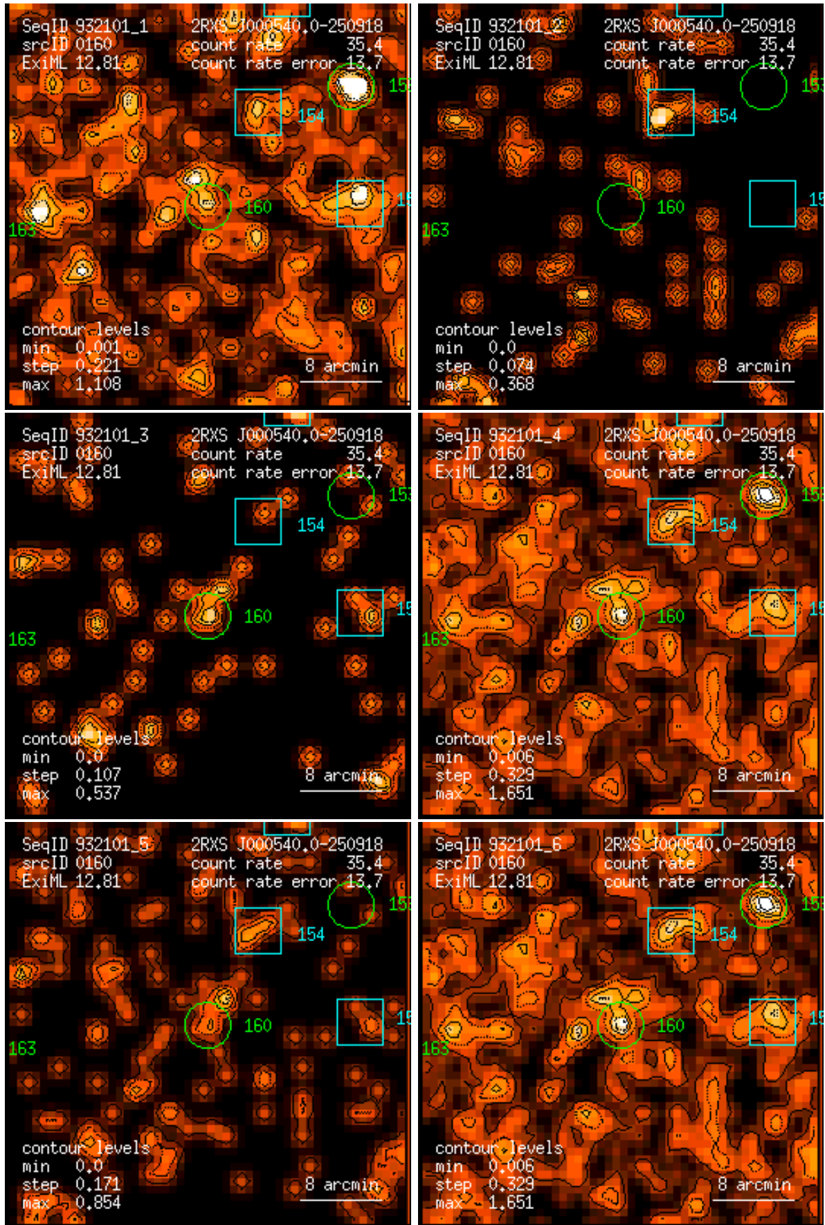
Figure 160: RASS 932101: detection 0160: band rate images, Gaussian filter: (1) PSPC channels 11 – 41, (2) 52 – 90, (3) 91 – 201, (4) 11 – 235, (5) 52 – 201, (6) 11 – 201. Broad band rates in counts/ks. Band rate contour levels in counts/ks/arcmin 2 .
