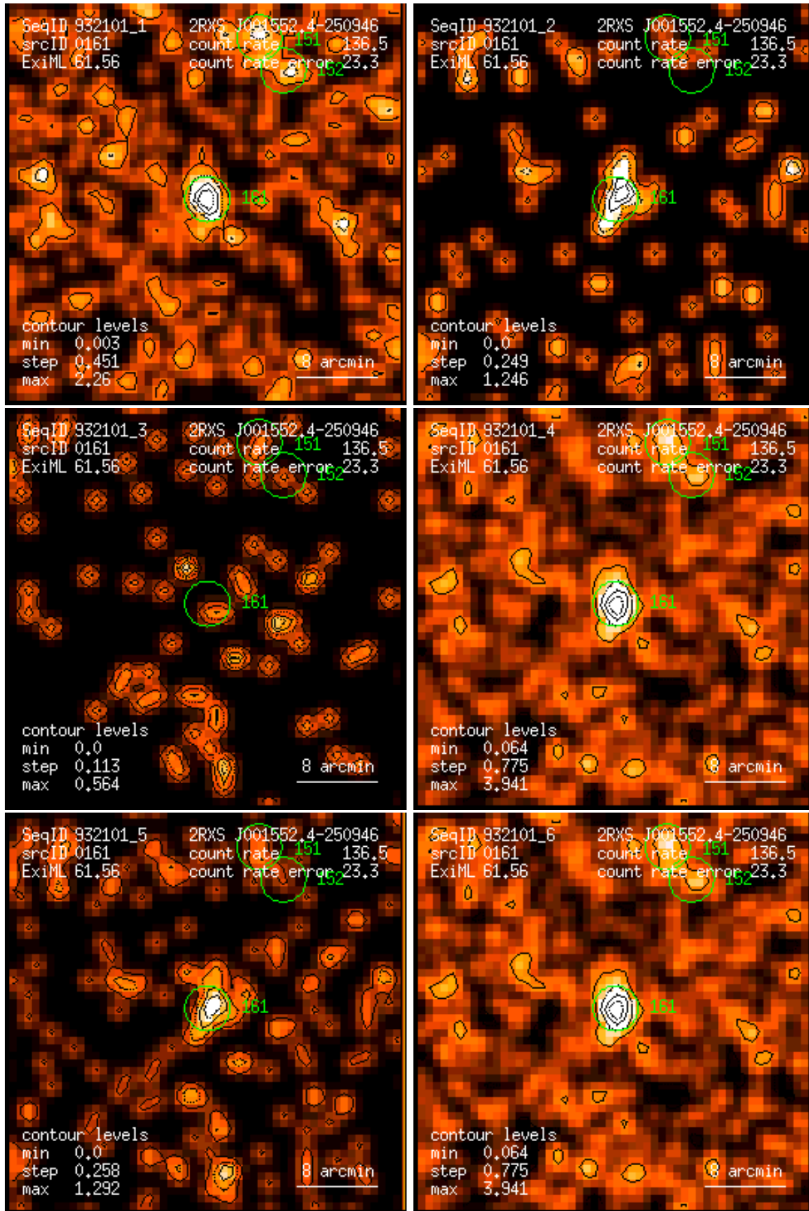
Figure 161: RASS 932101: detection 0161: band rate images, Gaussian filter: (1) PSPC channels 11 – 41, (2) 52 – 90, (3) 91 – 201, (4) 11 – 235, (5) 52 – 201, (6) 11 – 201. Broad band rates in counts/ks. Band rate contour levels in counts/ks/arcmin 2 .
