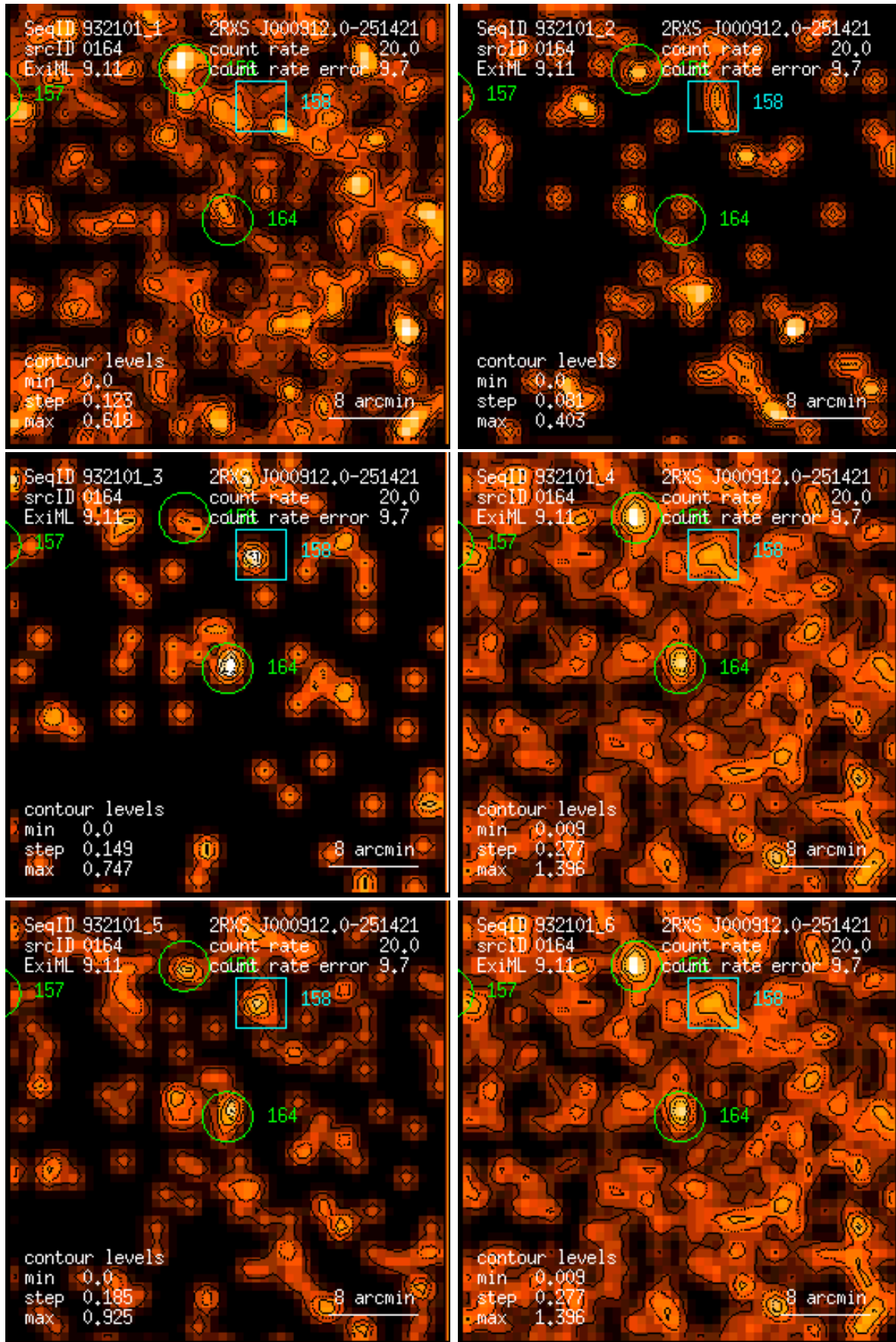
Figure 164: RASS 932101: detection 0164: band rate images, Gaussian filter: (1) PSPC channels 11 – 41, (2) 52 – 90, (3) 91 – 201, (4) 11 – 235, (5) 52 – 201, (6) 11 – 201. Broad band rates in counts/ks. Band rate contour levels in counts/ks/arcmin 2 .
