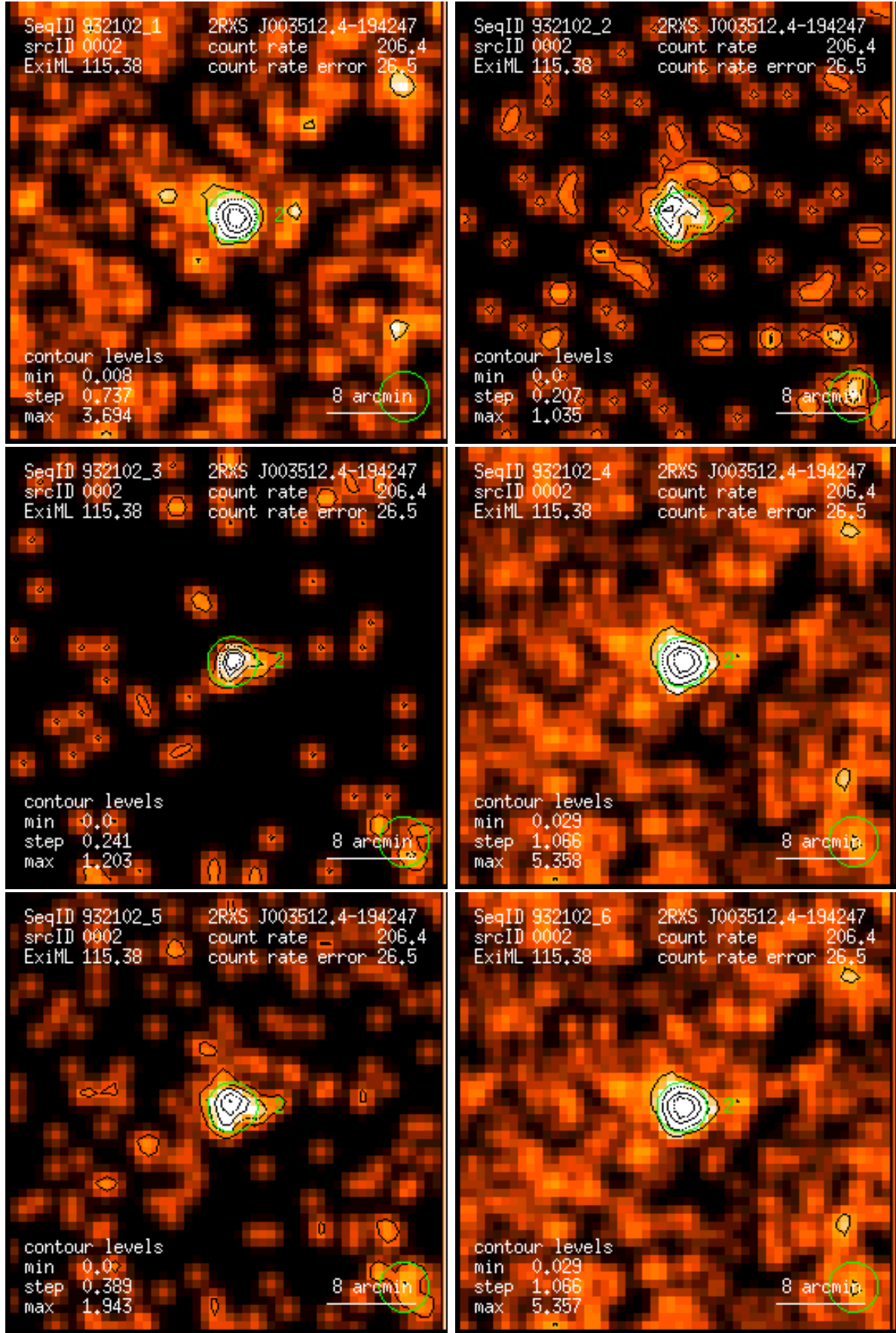
Figure 2: RASS 932102: detection 0002: band rate images, Gaussian filter: (1) PSPC channels 11 – 41, (2) 52 – 90, (3) 91 – 201, (4) 11 – 235, (5) 52 – 201, (6) 11 – 201. Broad band rates in counts/ks. Band rate contour levels in counts/ks/arcmin 2 .
