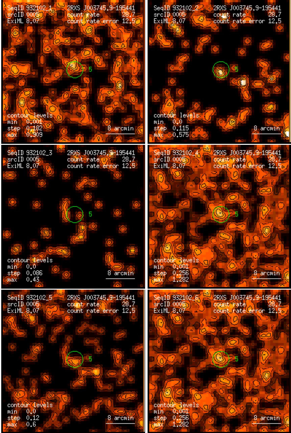
Figure 5: RASS 932102: detection 0005: band rate images, Gaussian filter: (1) PSPC channels 11 – 41, (2) 52 – 90, (3) 91 – 201, (4) 11 – 235, (5) 52 – 201, (6) 11 – 201. Broad band rates in counts/ks. Band rate contour levels in counts/ks/arcmin 2 .
