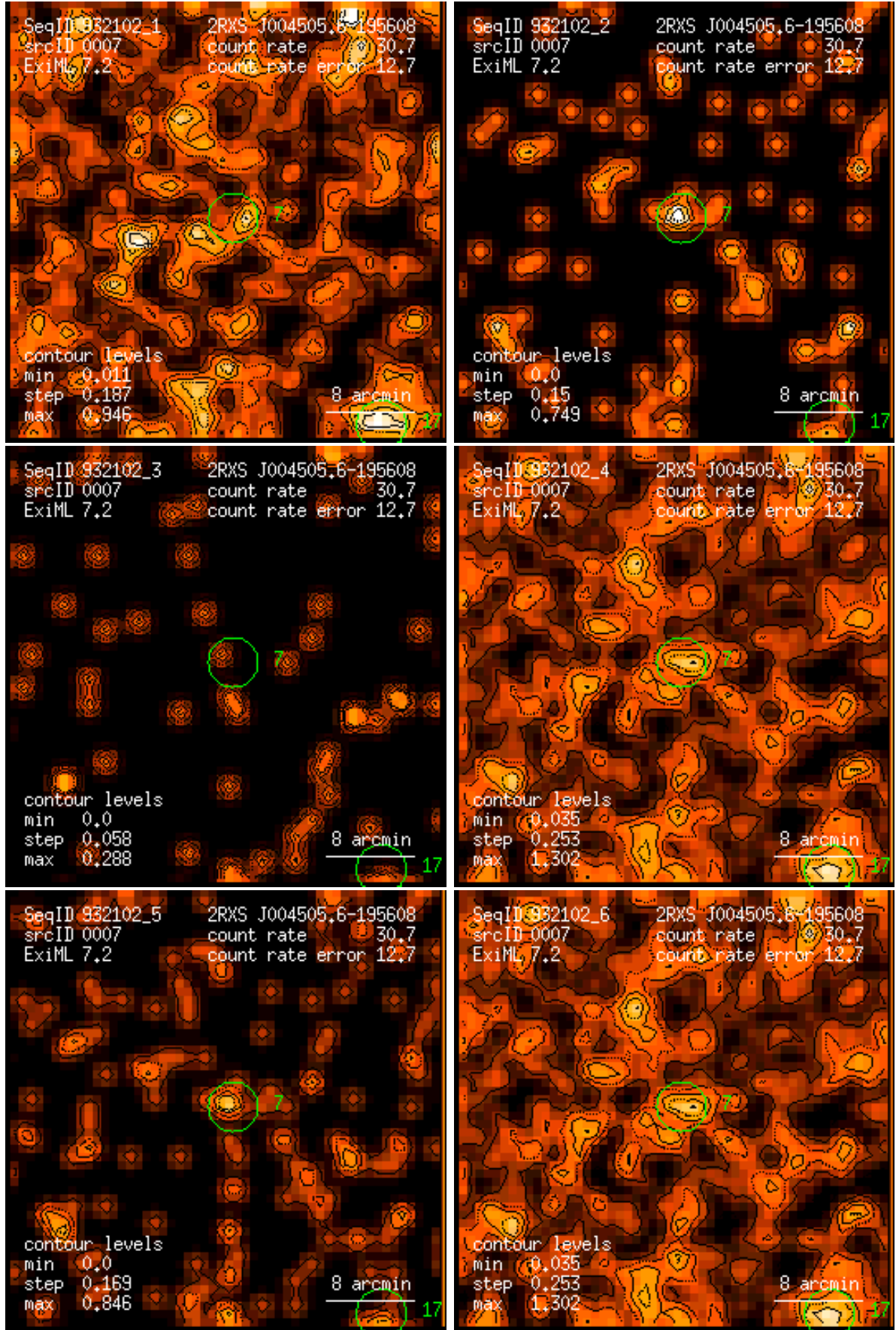
Figure 7: RASS 932102: detection 0007: band rate images, Gaussian filter: (1) PSPC channels 11 – 41, (2) 52 – 90, (3) 91 – 201, (4) 11 – 235, (5) 52 – 201, (6) 11 – 201. Broad band rates in counts/ks. Band rate contour levels in counts/ks/arcmin 2 .
