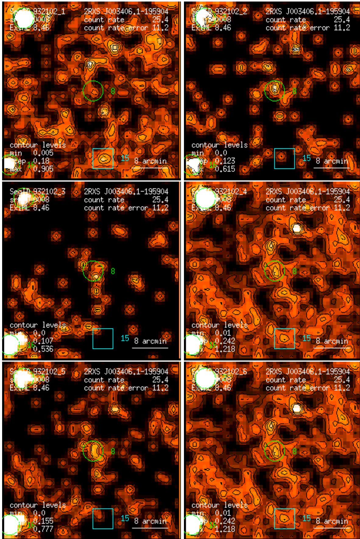
Figure 8: RASS 932102: detection 0008: band rate images, Gaussian filter: (1) PSPC channels 11 – 41, (2) 52 – 90, (3) 91 – 201, (4) 11 – 235, (5) 52 – 201, (6) 11 – 201. Broad band rates in counts/ks. Band rate contour levels in counts/ks/arcmin 2 .
