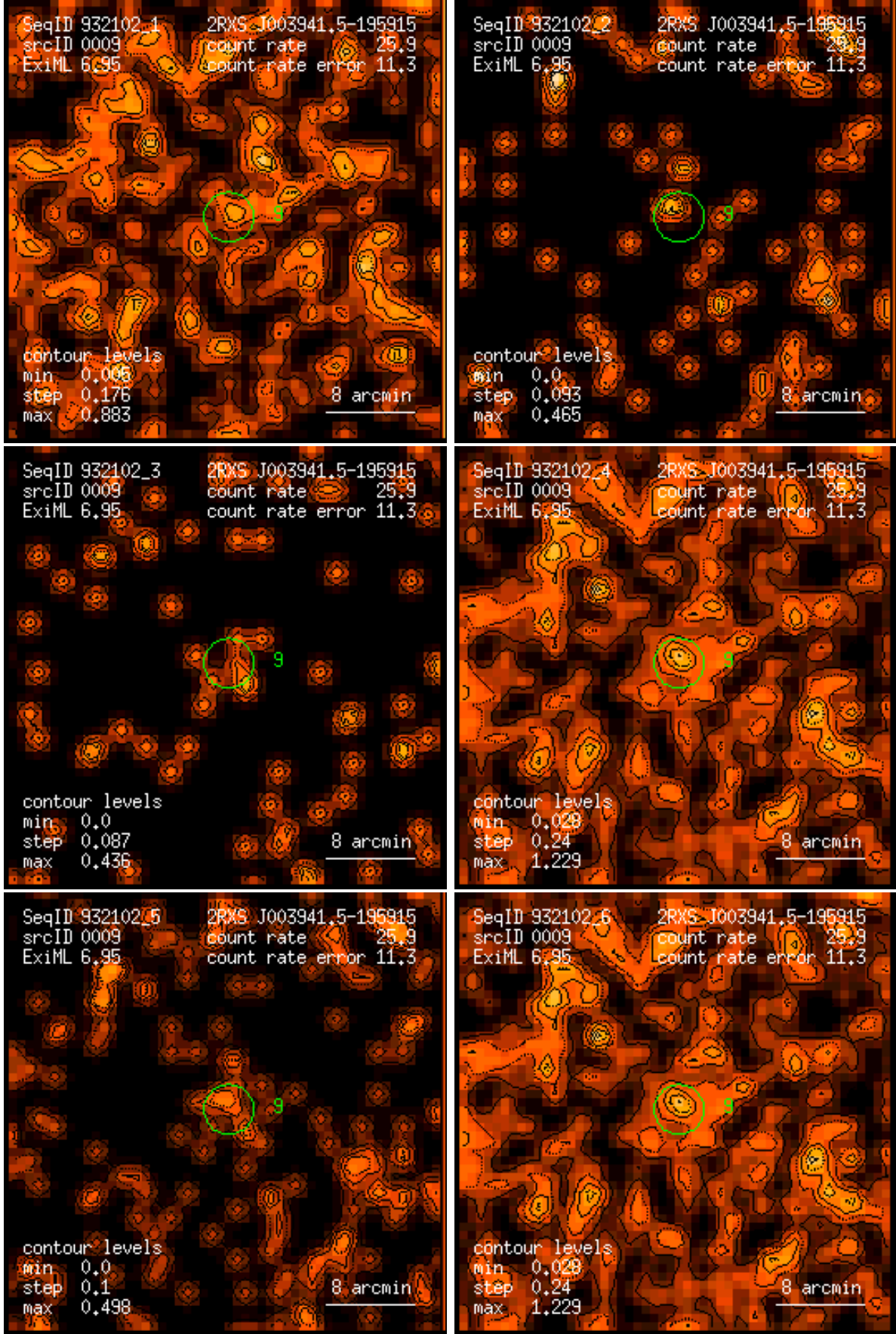
Figure 9: RASS 932102: detection 0009: band rate images, Gaussian filter: (1) PSPC channels 11 – 41, (2) 52 – 90, (3) 91 – 201, (4) 11 – 235, (5) 52 – 201, (6) 11 – 201. Broad band rates in counts/ks. Band rate contour levels in counts/ks/arcmin 2 .
