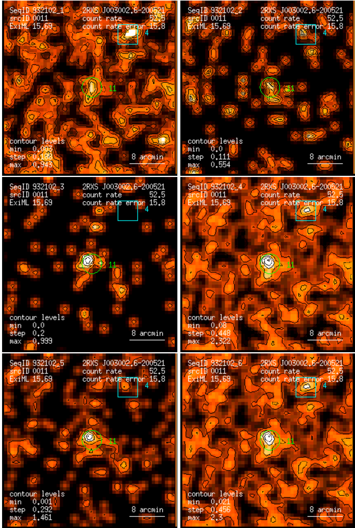
Figure 11: RASS 932102: detection 0011: band rate images, Gaussian filter: (1) PSPC channels 11 – 41, (2) 52 – 90, (3) 91 – 201, (4) 11 – 235, (5) 52 – 201, (6) 11 – 201. Broad band rates in counts/ks. Band rate contour levels in counts/ks/arcmin 2 .
