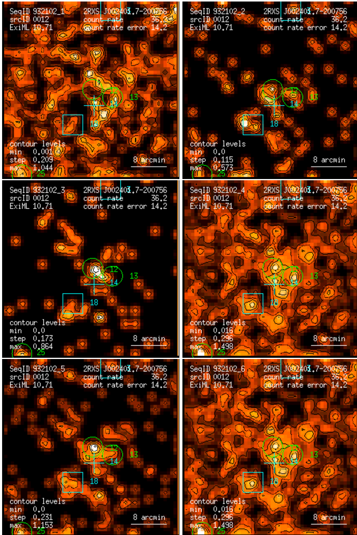
Figure 12: RASS 932102: detection 0012: band rate images, Gaussian filter: (1) PSPC channels 11 – 41, (2) 52 – 90, (3) 91 – 201, (4) 11 – 235, (5) 52 – 201, (6) 11 – 201. Broad band rates in counts/ks. Band rate contour levels in counts/ks/arcmin 2 .
