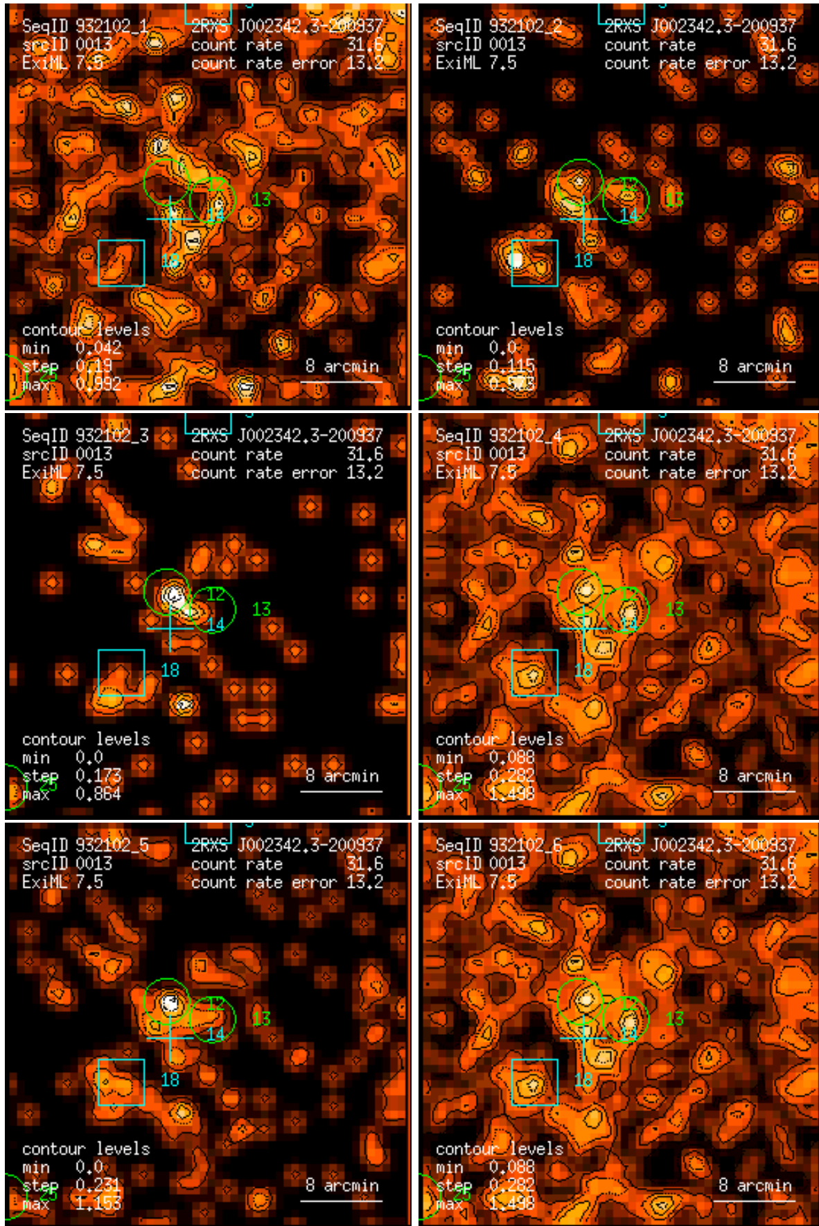
Figure 13: RASS 932102: detection 0013: band rate images, Gaussian filter: (1) PSPC channels 11 – 41, (2) 52 – 90, (3) 91 – 201, (4) 11 – 235, (5) 52 – 201, (6) 11 – 201. Broad band rates in counts/ks. Band rate contour levels in counts/ks/arcmin 2 .
