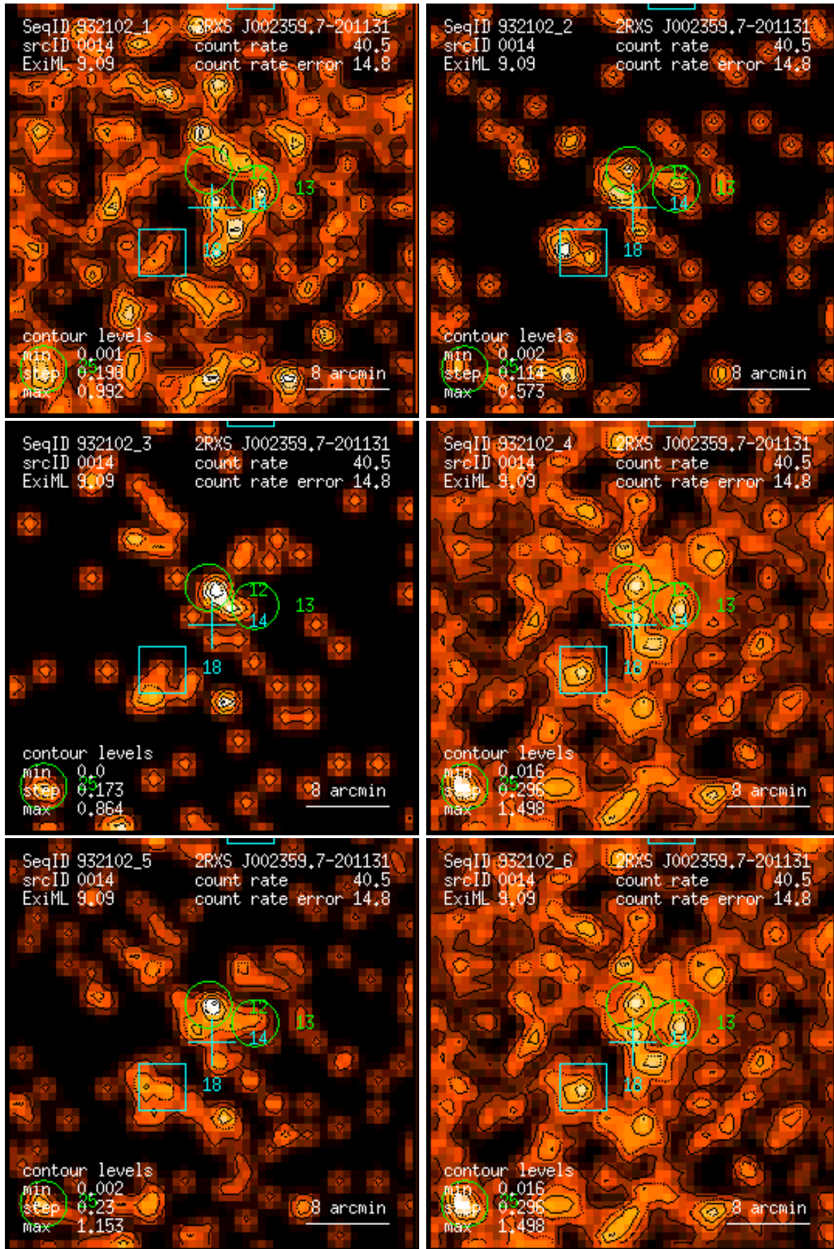
Figure 14: RASS 932102: detection 0014: band rate images, Gaussian filter: (1) PSPC channels 11 – 41, (2) 52 – 90, (3) 91 – 201, (4) 11 – 235, (5) 52 – 201, (6) 11 – 201. Broad band rates in counts/ks. Band rate contour levels in counts/ks/arcmin 2 .
