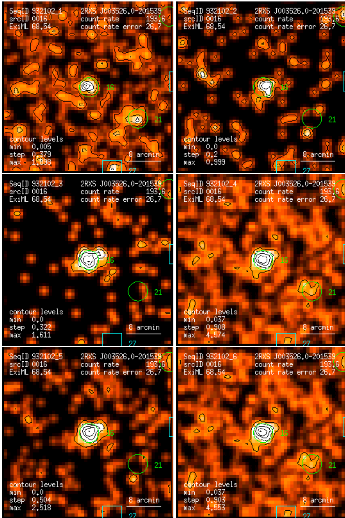
Figure 16: RASS 932102: detection 0016: band rate images, Gaussian filter: (1) PSPC channels 11 – 41, (2) 52 – 90, (3) 91 – 201, (4) 11 – 235, (5) 52 – 201, (6) 11 – 201. Broad band rates in counts/ks. Band rate contour levels in counts/ks/arcmin 2 .
