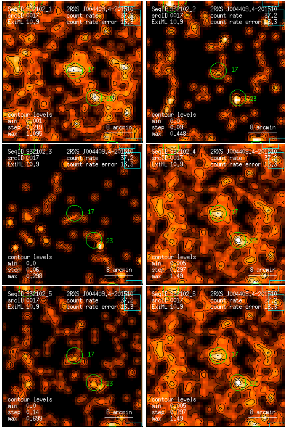
Figure 17: RASS 932102: detection 0017: band rate images, Gaussian filter: (1) PSPC channels 11 – 41, (2) 52 – 90, (3) 91 – 201, (4) 11 – 235, (5) 52 – 201, (6) 11 – 201. Broad band rates in counts/ks. Band rate contour levels in counts/ks/arcmin 2 .
