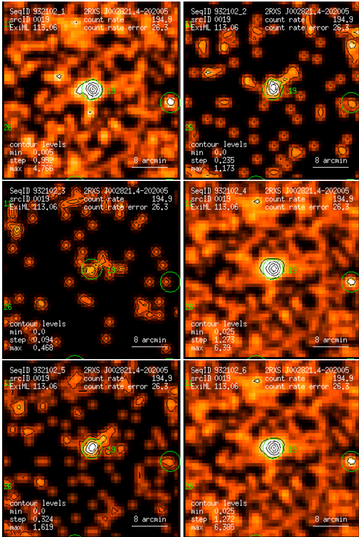
Figure 19: RASS 932102: detection 0019: band rate images, Gaussian filter: (1) PSPC channels 11 – 41, (2) 52 – 90, (3) 91 – 201, (4) 11 – 235, (5) 52 – 201, (6) 11 – 201. Broad band rates in counts/ks. Band rate contour levels in counts/ks/arcmin 2 .
