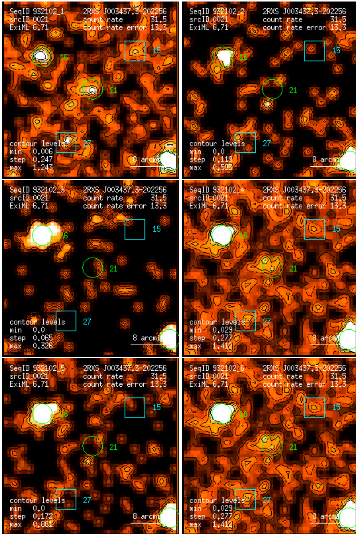
Figure 21: RASS 932102: detection 0021: band rate images, Gaussian filter: (1) PSPC channels 11 – 41, (2) 52 – 90, (3) 91 – 201, (4) 11 – 235, (5) 52 – 201, (6) 11 – 201. Broad band rates in counts/ks. Band rate contour levels in counts/ks/arcmin 2 .
