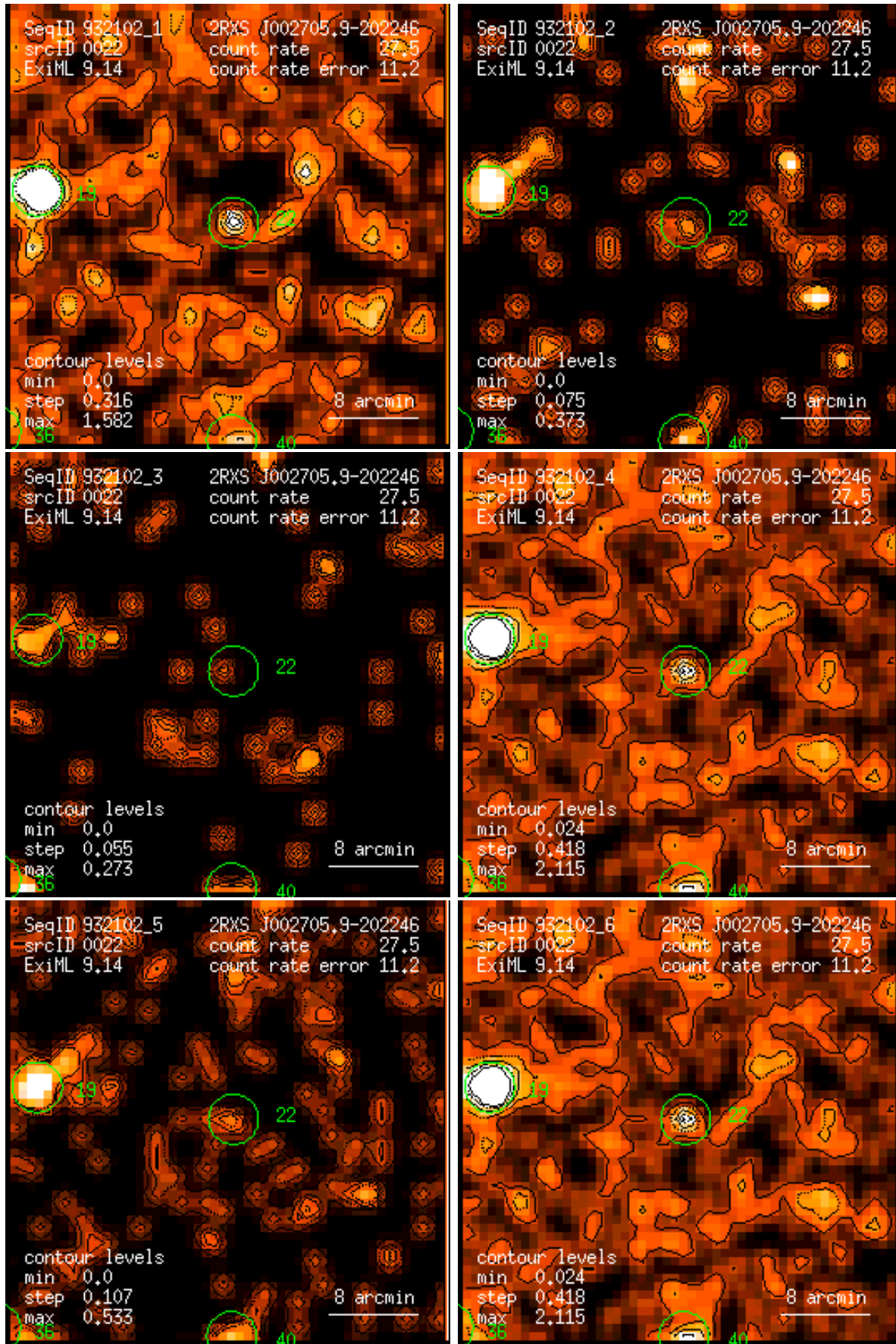
Figure 22: RASS 932102: detection 0022: band rate images, Gaussian filter: (1) PSPC channels 11 – 41, (2) 52 – 90, (3) 91 – 201, (4) 11 – 235, (5) 52 – 201, (6) 11 – 201. Broad band rates in counts/ks. Band rate contour levels in counts/ks/arcmin 2 .
