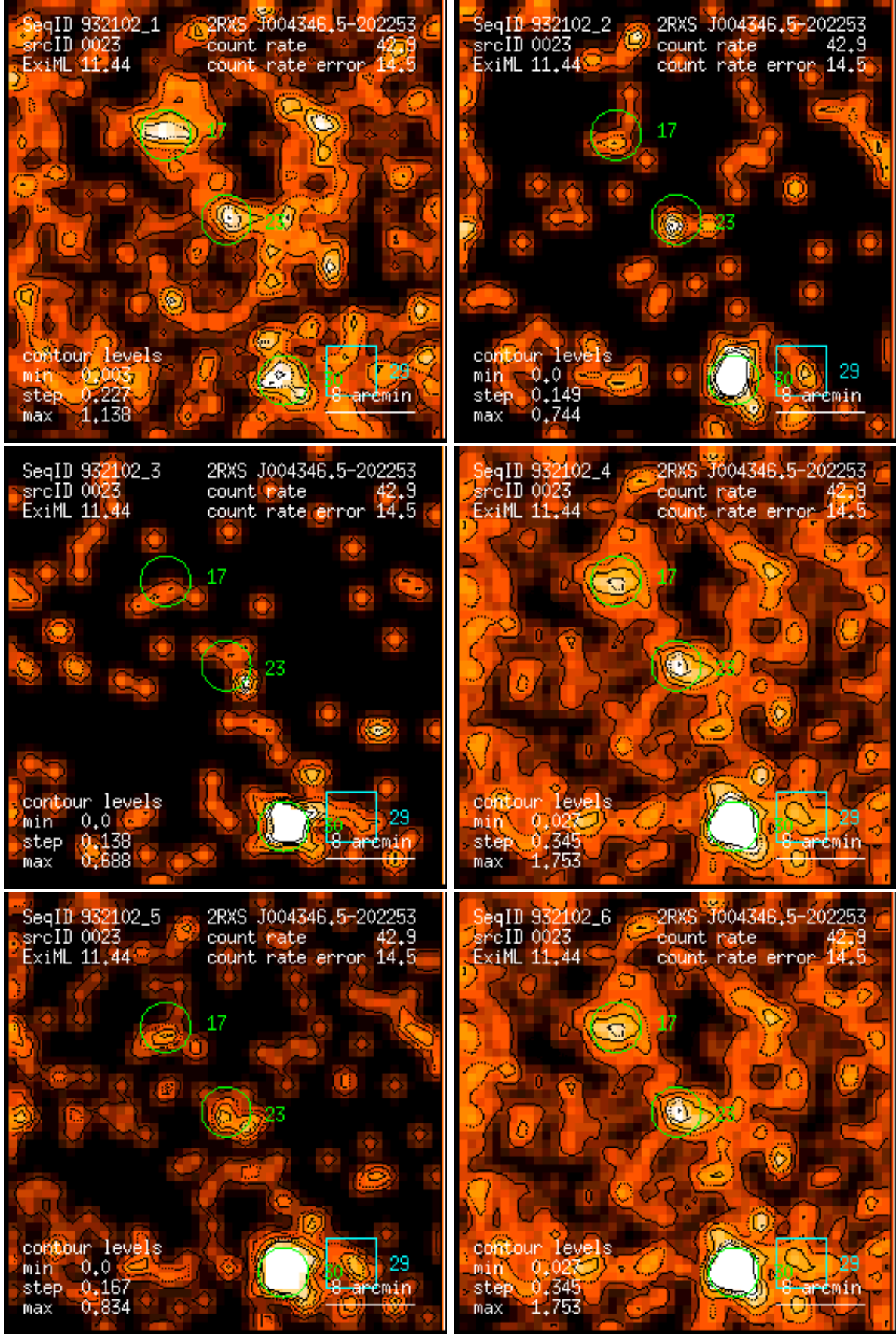
Figure 23: RASS 932102: detection 0023: band rate images, Gaussian filter: (1) PSPC channels 11 – 41, (2) 52 – 90, (3) 91 – 201, (4) 11 – 235, (5) 52 – 201, (6) 11 – 201. Broad band rates in counts/ks. Band rate contour levels in counts/ks/arcmin 2 .
