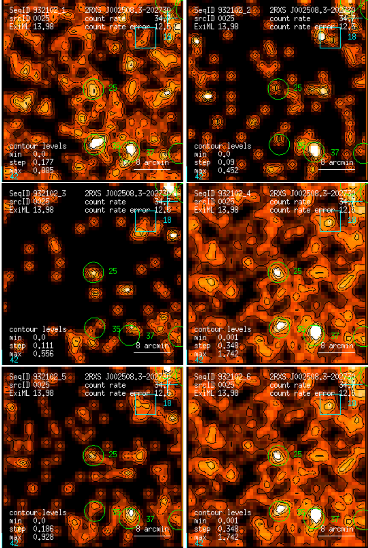
Figure 25: RASS 932102: detection 0025: band rate images, Gaussian filter: (1) PSPC channels 11 – 41, (2) 52 – 90, (3) 91 – 201, (4) 11 – 235, (5) 52 – 201, (6) 11 – 201. Broad band rates in counts/ks. Band rate contour levels in counts/ks/arcmin 2 .
