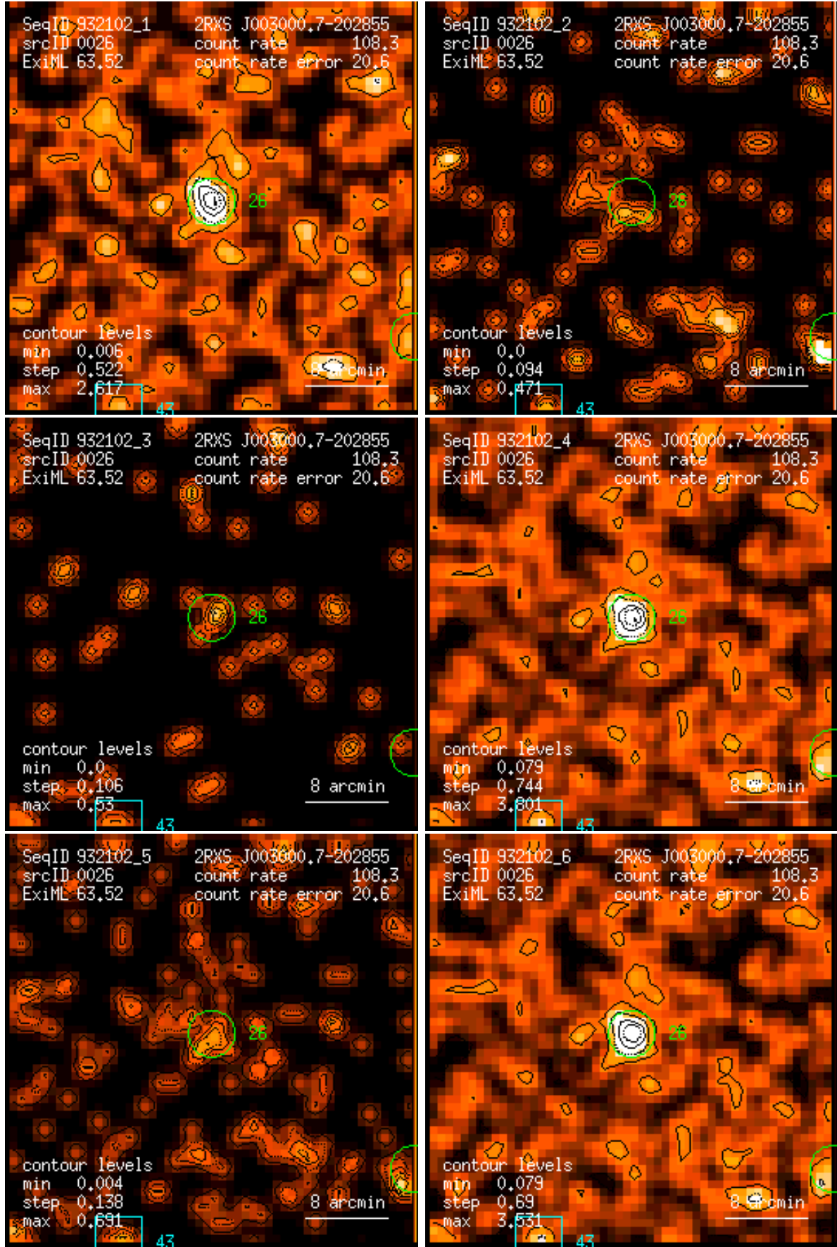
Figure 26: RASS 932102: detection 0026: band rate images, Gaussian filter: (1) PSPC channels 11 – 41, (2) 52 – 90, (3) 91 – 201, (4) 11 – 235, (5) 52 – 201, (6) 11 – 201. Broad band rates in counts/ks. Band rate contour levels in counts/ks/arcmin 2 .
