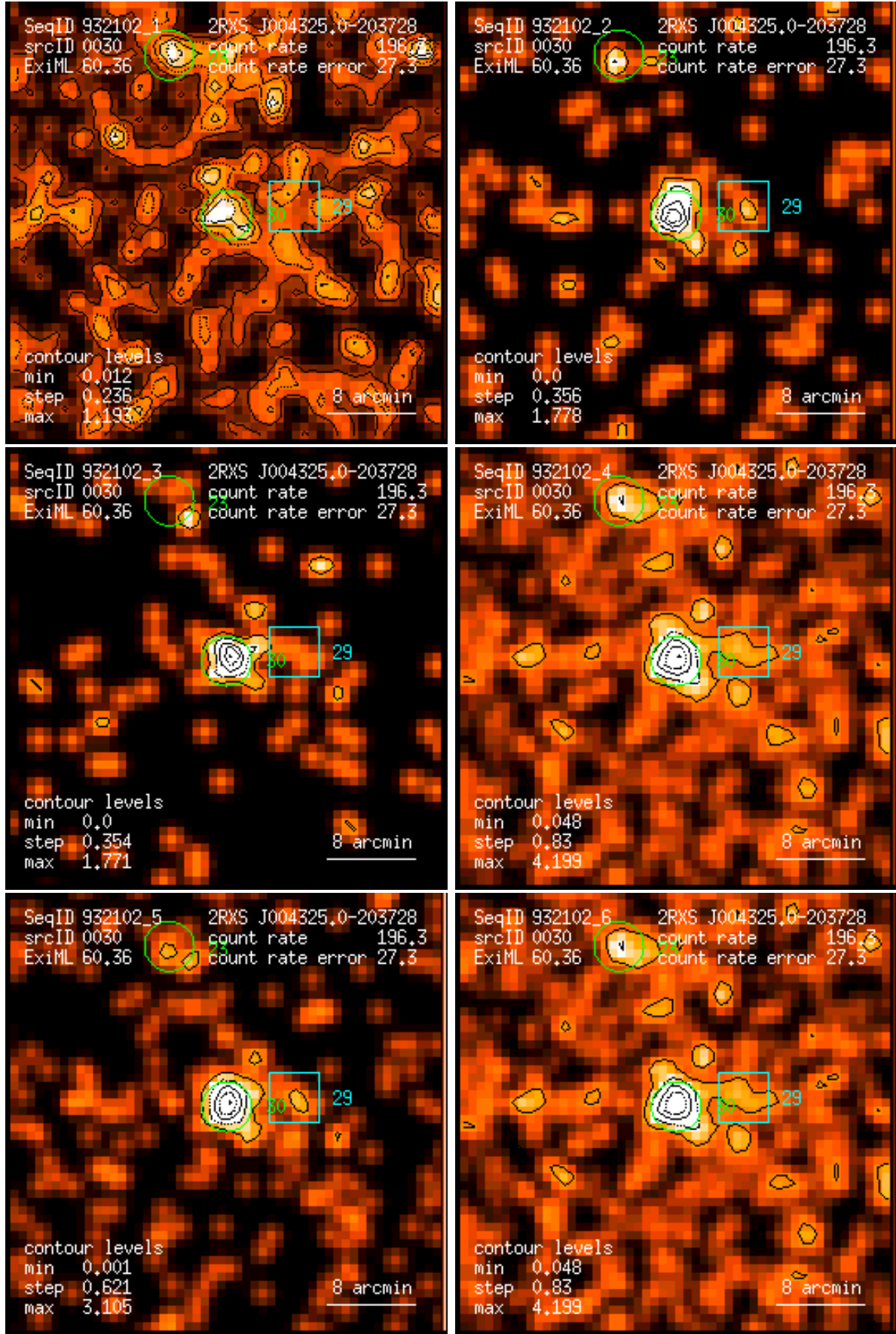
Figure 30: RASS 932102: detection 0030: band rate images, Gaussian filter: (1) PSPC channels 11 – 41, (2) 52 – 90, (3) 91 – 201, (4) 11 – 235, (5) 52 – 201, (6) 11 – 201. Broad band rates in counts/ks. Band rate contour levels in counts/ks/arcmin 2 .
