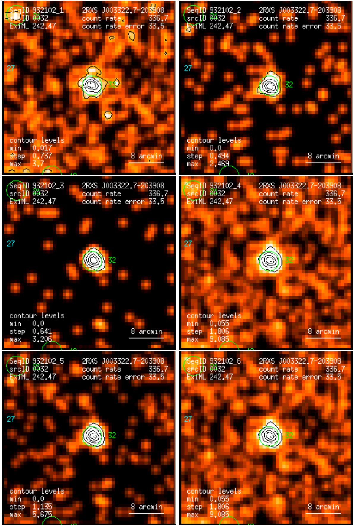
Figure 32: RASS 932102: detection 0032: band rate images, Gaussian filter: (1) PSPC channels 11 – 41, (2) 52 – 90, (3) 91 – 201, (4) 11 – 235, (5) 52 – 201, (6) 11 – 201. Broad band rates in counts/ks. Band rate contour levels in counts/ks/arcmin 2 .
