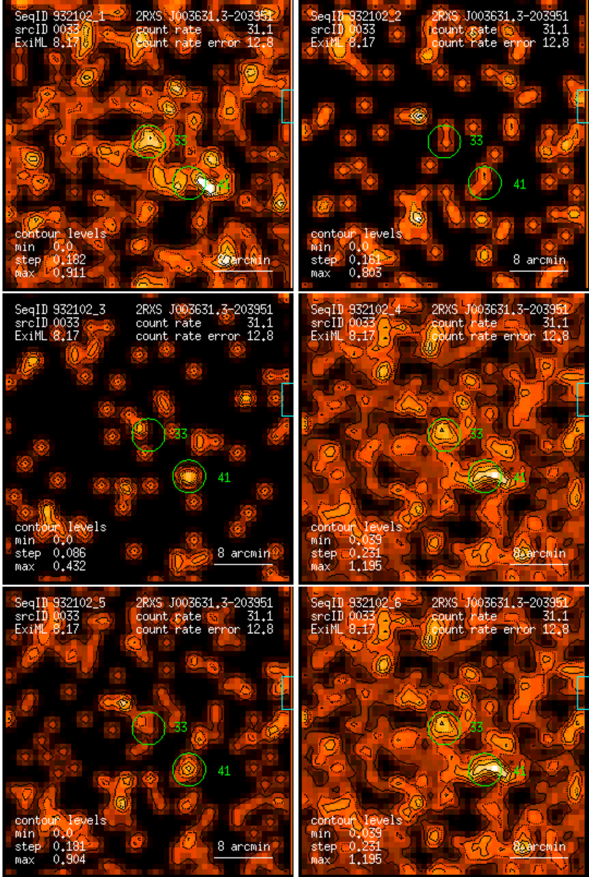
Figure 33: RASS 932102: detection 0033: band rate images, Gaussian filter: (1) PSPC channels 11 – 41, (2) 52 – 90, (3) 91 – 201, (4) 11 – 235, (5) 52 – 201, (6) 11 – 201. Broad band rates in counts/ks. Band rate contour levels in counts/ks/arcmin 2 .
