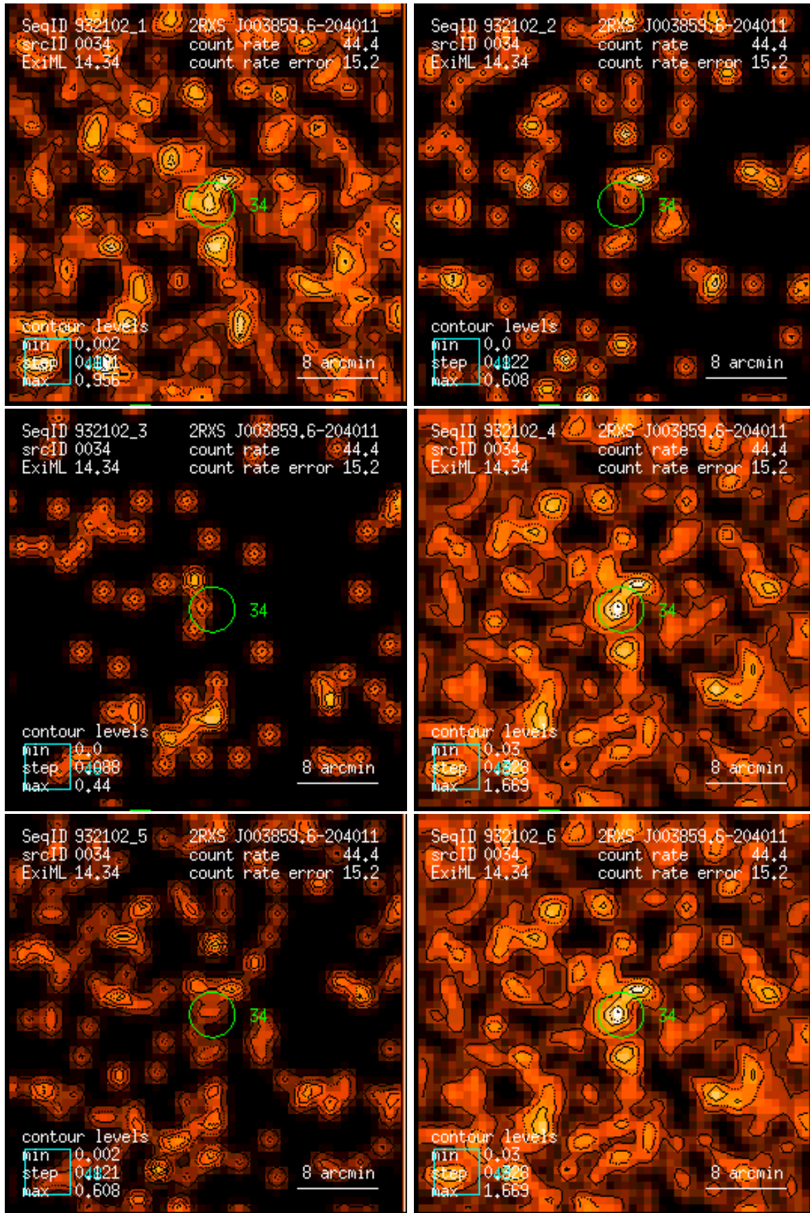
Figure 34: RASS 932102: detection 0034: band rate images, Gaussian filter: (1) PSPC channels 11 – 41, (2) 52 – 90, (3) 91 – 201, (4) 11 – 235, (5) 52 – 201, (6) 11 – 201. Broad band rates in counts/ks. Band rate contour levels in counts/ks/arcmin 2 .
