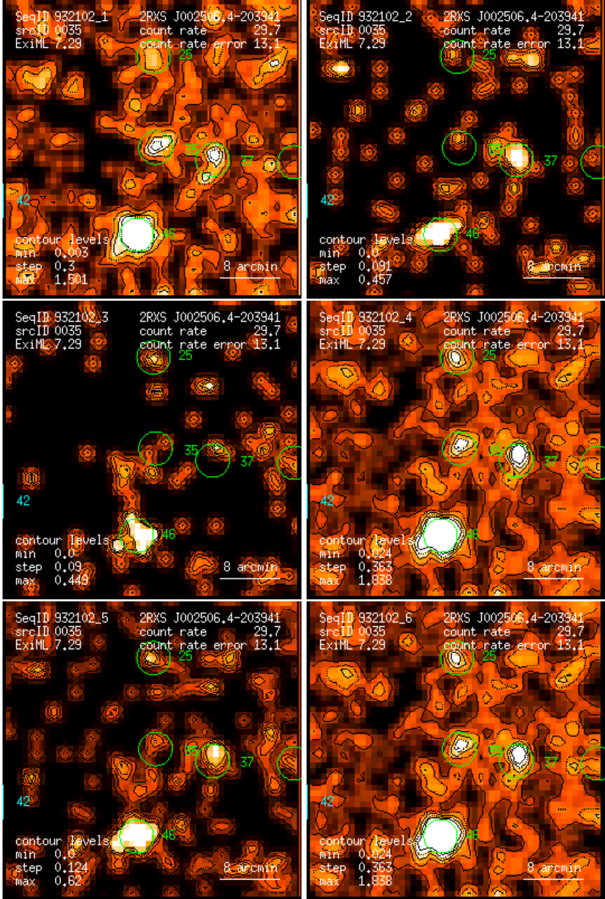
Figure 35: RASS 932102: detection 0035: band rate images, Gaussian filter: (1) PSPC channels 11 – 41, (2) 52 – 90, (3) 91 – 201, (4) 11 – 235, (5) 52 – 201, (6) 11 – 201. Broad band rates in counts/ks. Band rate contour levels in counts/ks/arcmin 2 .
