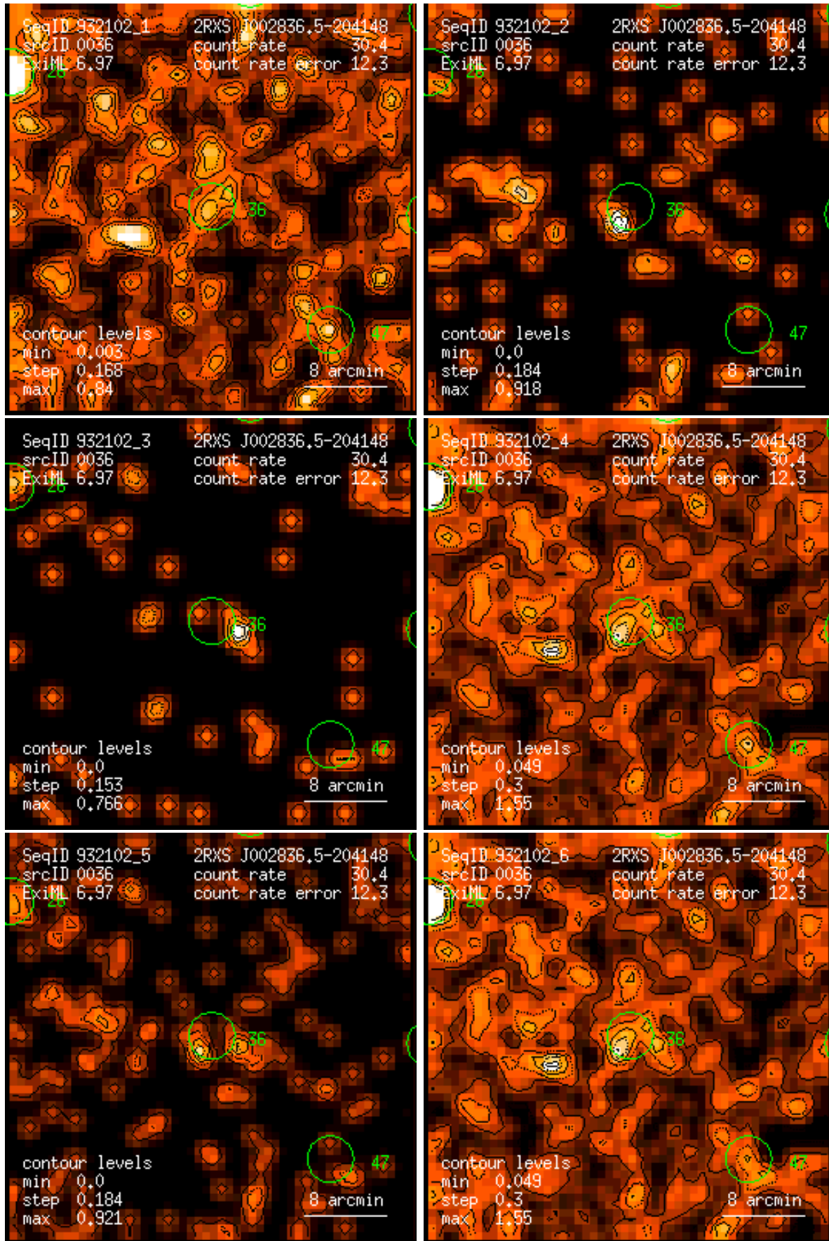
Figure 36: RASS 932102: detection 0036: band rate images, Gaussian filter: (1) PSPC channels 11 – 41, (2) 52 – 90, (3) 91 – 201, (4) 11 – 235, (5) 52 – 201, (6) 11 – 201. Broad band rates in counts/ks. Band rate contour levels in counts/ks/arcmin 2 .
