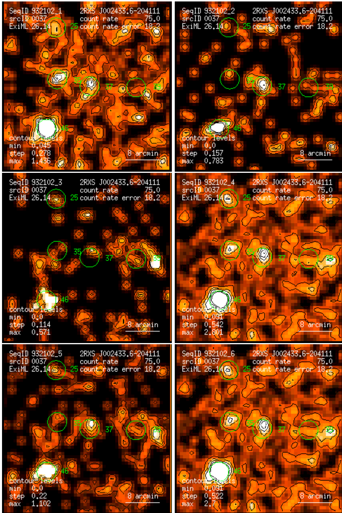
Figure 37: RASS 932102: detection 0037: band rate images, Gaussian filter: (1) PSPC channels 11 – 41, (2) 52 – 90, (3) 91 – 201, (4) 11 – 235, (5) 52 – 201, (6) 11 – 201. Broad band rates in counts/ks. Band rate contour levels in counts/ks/arcmin 2 .
