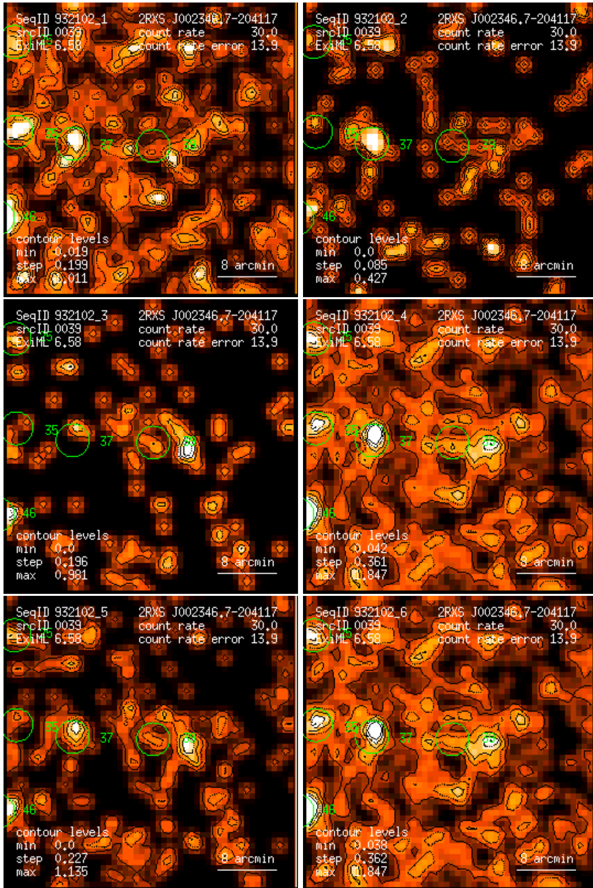
Figure 39: RASS 932102: detection 0039: band rate images, Gaussian filter: (1) PSPC channels 11 – 41, (2) 52 – 90, (3) 91 – 201, (4) 11 – 235, (5) 52 – 201, (6) 11 – 201. Broad band rates in counts/ks. Band rate contour levels in counts/ks/arcmin 2 .
