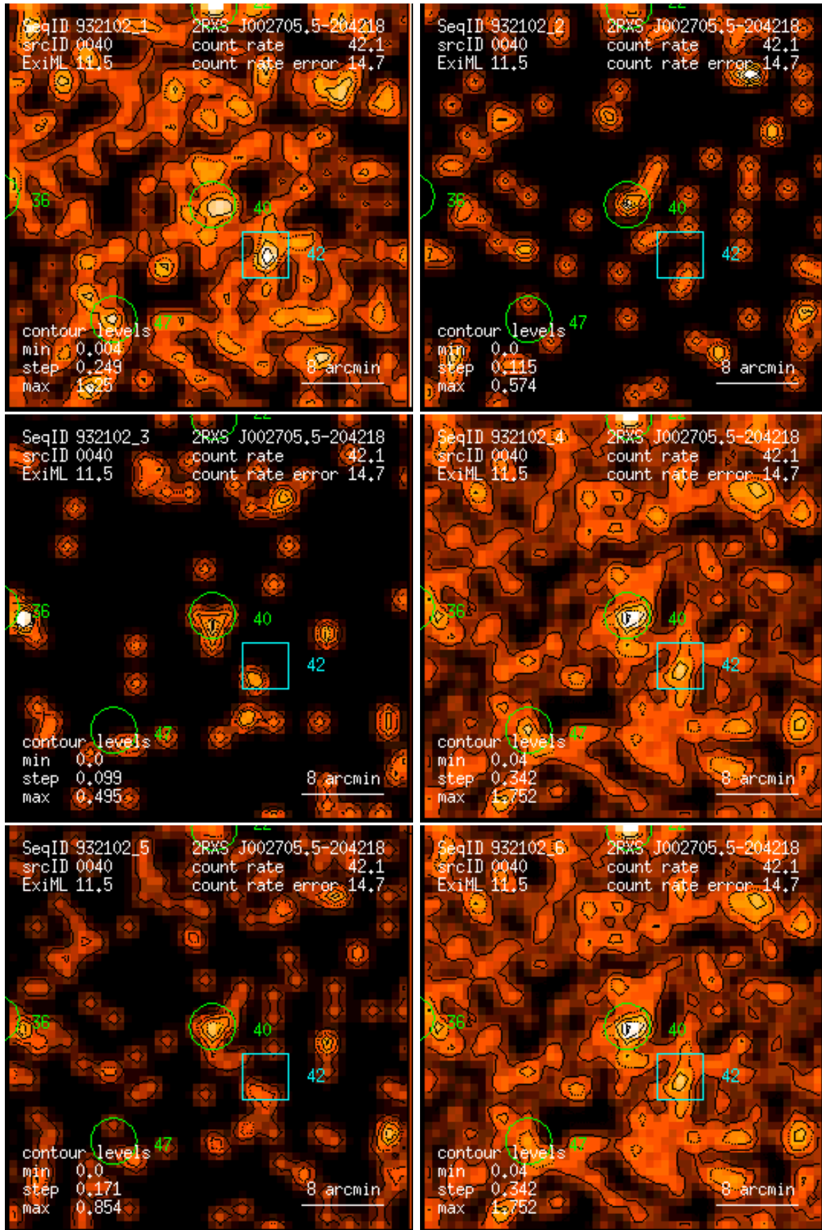
Figure 40: RASS 932102: detection 0040: band rate images, Gaussian filter: (1) PSPC channels 11 – 41, (2) 52 – 90, (3) 91 – 201, (4) 11 – 235, (5) 52 – 201, (6) 11 – 201. Broad band rates in counts/ks. Band rate contour levels in counts/ks/arcmin 2 .
