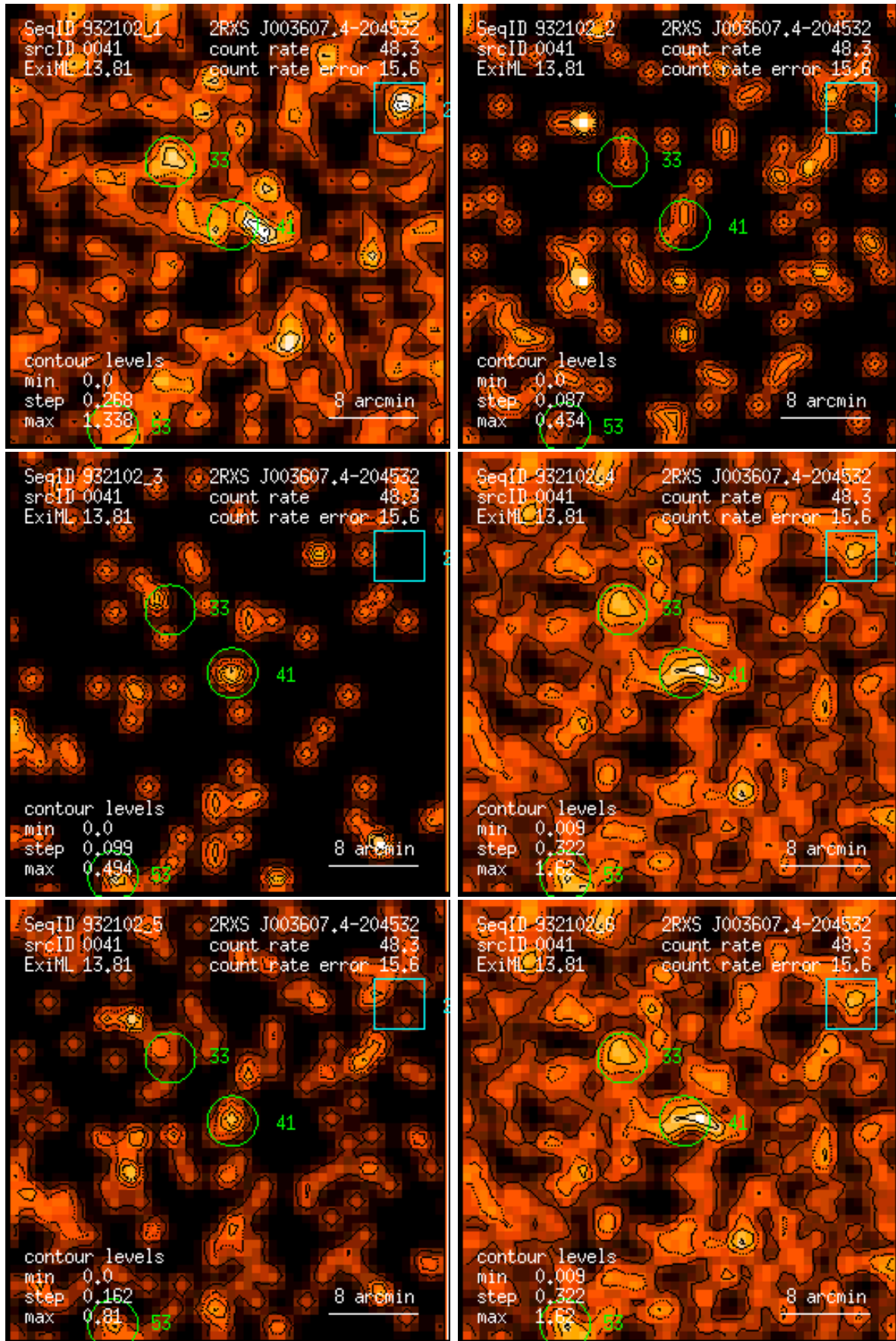
Figure 41: RASS 932102: detection 0041: band rate images, Gaussian filter: (1) PSPC channels 11 – 41, (2) 52 – 90, (3) 91 – 201, (4) 11 – 235, (5) 52 – 201, (6) 11 – 201. Broad band rates in counts/ks. Band rate contour levels in counts/ks/arcmin 2 .
