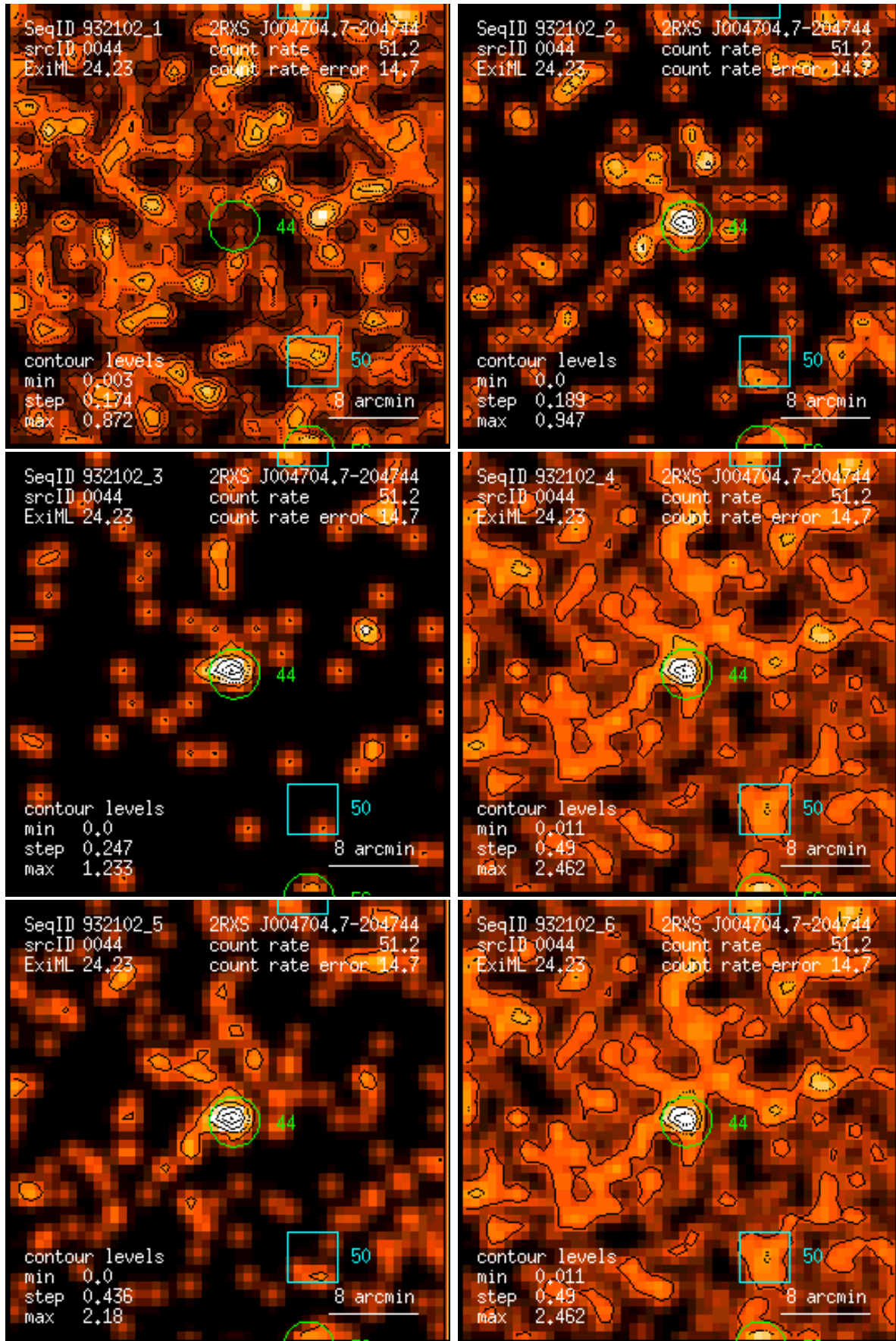
Figure 44: RASS 932102: detection 0044: band rate images, Gaussian filter: (1) PSPC channels 11 – 41, (2) 52 – 90, (3) 91 – 201, (4) 11 – 235, (5) 52 – 201, (6) 11 – 201. Broad band rates in counts/ks. Band rate contour levels in counts/ks/arcmin 2 .
