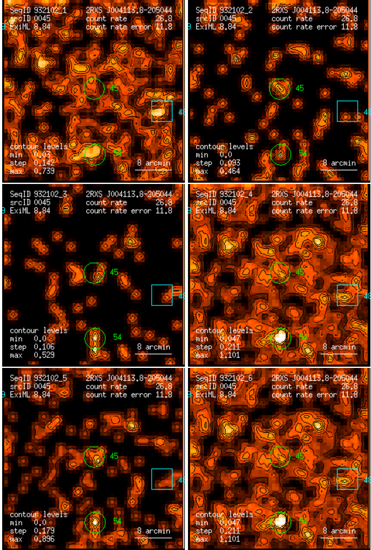
Figure 45: RASS 932102: detection 0045: band rate images, Gaussian filter: (1) PSPC channels 11 – 41, (2) 52 – 90, (3) 91 – 201, (4) 11 – 235, (5) 52 – 201, (6) 11 – 201. Broad band rates in counts/ks. Band rate contour levels in counts/ks/arcmin 2 .
